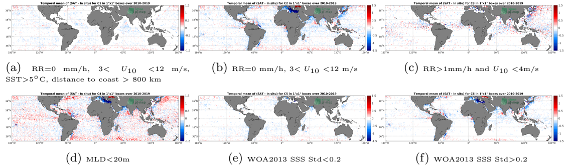
Figure 12: Temporal mean gridded over spatial boxes of size 1^\circ \times 1^\circ of \Delta SSS (SMOS-L3-CATDS-CPDC-V3-MONTHLY-25KM - Argo) for 6 different subdatasets corresponding to: RR=0 mm/h, 3 < U_{10} < 12 m/s, SST > 5^\circ\text{C} , distance to coast > 800 km (a), RR=0 mm/h, 3 < U_{10} < 12 m/s (b), RR > 1 mm/h and U_{10} < 4 m/s (c), MLD < 20 m (d), WOA2013 SSS Std < 0.2 (e), WOA2013 SSS Std > 0.2 (f).
