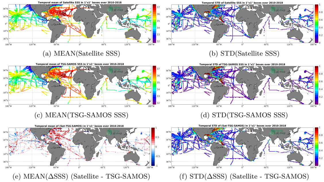
Figure 6: Temporal mean (left) and STD (right) of SSS from SMOS-L3-CATDS-CPDC-V3-10DAYS-25KM (top), TSG-SAMOS (middle), and of \Delta SSS (Satellite - TSG-SAMOS). Only match-up pairs are used to generate these maps.
