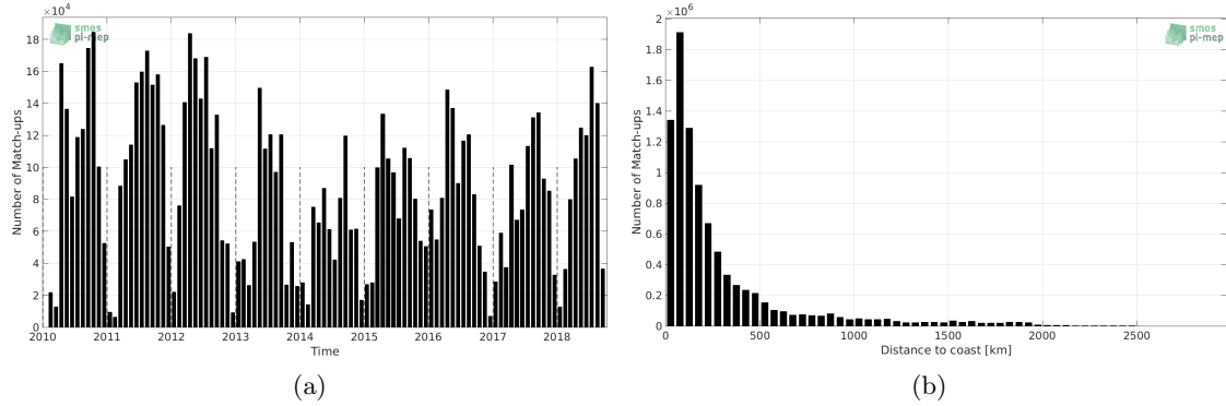
Figure 1: Number of match-ups between TSG-SAMOS and SMOS-L3-CATDS-CPDC-V3-10DAYS-25KM SSS as a function of time (a) and as function of the distance to coast (b) over the Mid-Low Latitudes 45N-45S Pi-MEP region and for the full satellite product period.
