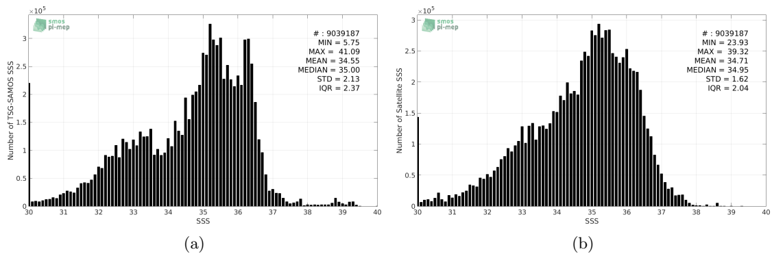
Figure 2: Histograms of SSS from TSG-SAMOS (a) and SMOS-L3-CATDS-CPDC-V3-10DAYS-25KM (b) considering all match-up pairs per bins of 0.1 over the Mid-Low Latitudes 45N-45S Pi-MEP region and for the full satellite product period.
