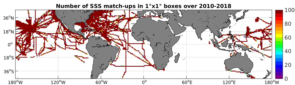
Figure 4: Number of SSS match-ups between TSG-SAMOS SSS and the SMOS-L3-CATDS-CPDC-V3-10DAYS-25KM SSS product for the Mid-Low Latitudes 45N-45S Pi-MEP region over 1^\circ \times 1^\circ boxes and for the full satellite product period.
