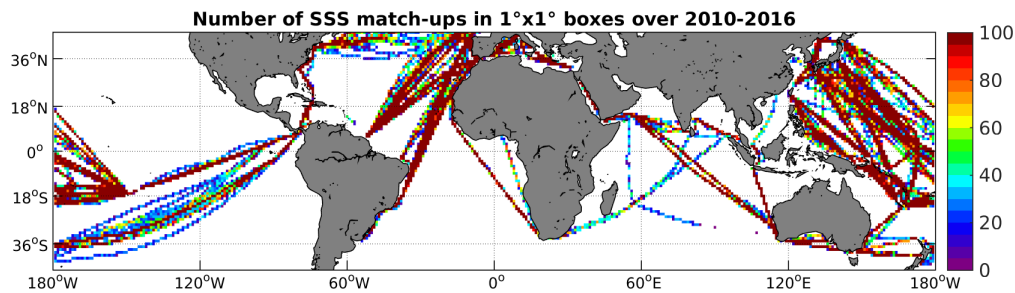
Figure 4: Number of SSS match-ups between TSG-LEGOS-DM SSS and the SMOS-L3-CATDS-CPDC-V3-10DAYS-25KM SSS product for the Mid-Low Latitudes 45N-45S Pi-MEP region over 1°x1° boxes and for the full satellite product period.
