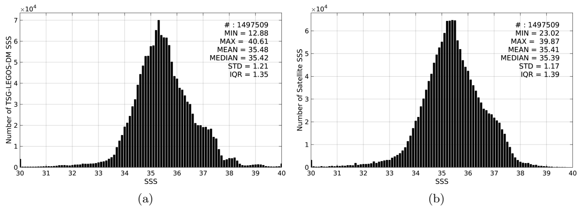
Figure 2: Histograms of SSS from TSG-LEGOS-DM (a) and SMOS-L3-CATDS-CPDC-V3-10DAYS-25KM (b) considering all match-up pairs per bins of 0.1 over the Mid-Low Latitudes 45N-45S Pi-MEP region and for the full satellite product period.
