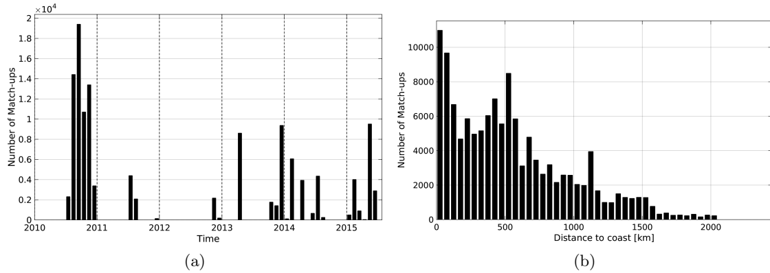
Figure 1: Number of match-ups between TSG-GOSUD-Sailing-ship and SMOS-L3-CATDS-CPDC-V3-10DAYS-25KM SSS as a function of time (a) and as function of the distance to coast (b) over the Mid-Low Latitudes 45N-45S Pi-MEP region and for the full satellite product period.
