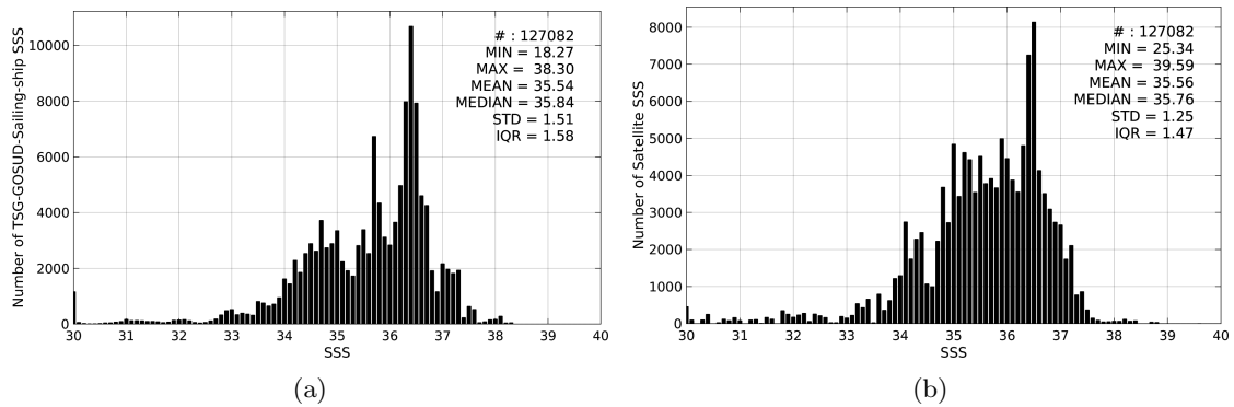
Figure 2: Histograms of SSS from TSG-GOSUD-Sailing-ship (a) and SMOS-L3-CATDS-CPDC-V3-10DAYS-25KM (b) considering all match-up pairs per bins of 0.1 over the Mid-Low Latitudes 45N-45S Pi-MEP region and for the full satellite product period.
