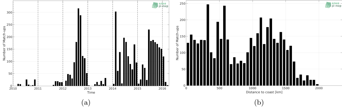
Figure 1: Number of match-ups between Sea mammals and SMOS-L3-CATDS-CPDC-V3-10DAYS-25KM SSS as a function of time (a) and as function of the distance to coast (b) over the Mid-Low Latitudes 45N-45S Pi-MEP region and for the full satellite product period.
