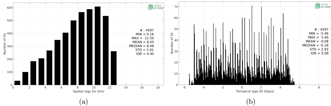
Figure 5: Histograms of the spatial (a) and temporal (b) lags between the time of the Sea mammals measurements and the date of the corresponding SMOS-L3-CATDS-CPDC-V3-10DAYS-25KM SSS product.
