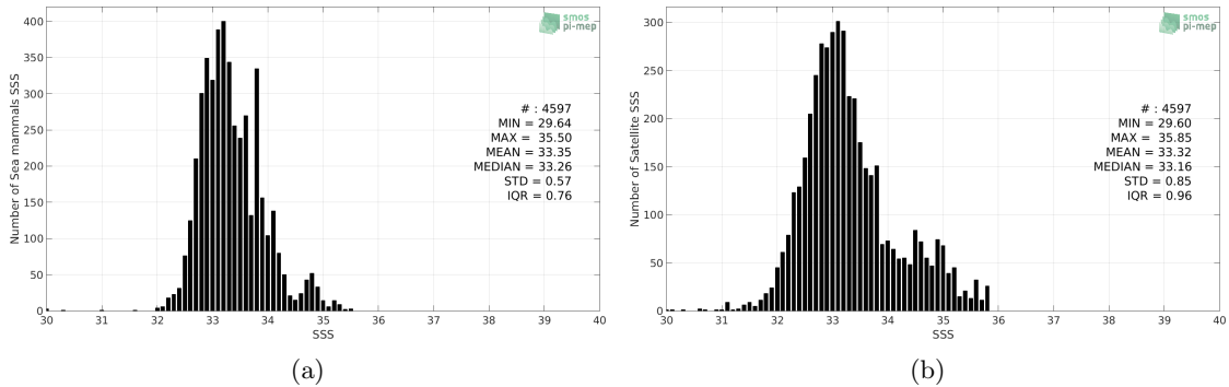
Figure 2: Histograms of SSS from Sea mammals (a) and SMOS-L3-CATDS-CPDC-V3-10DAYS-25KM (b) considering all match-up pairs per bins of 0.1 over the Mid-Low Latitudes 45N-45S Pi-MEP region and for the full satellite product period.
