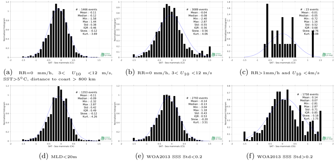
Figure 13: Normalized histogram of \Delta SSS (SMOS-L3-CATDS-CPDC-V3-10DAYS-25KM - Sea mammals) for 6 different subdatasets corresponding to: RR=0 mm/h, 3 < U_{10} < 12 m/s, SST>5°C, distance to coast > 800 km (a), RR=0 mm/h, 3 < U_{10} < 12 m/s (b), RR>1mm/h and U_{10} < 4 m/s (c), MLD<20m (d), WOA2013 SSS Std<0.2 (e), WOA2013 SSS Std>0.2 (f).
