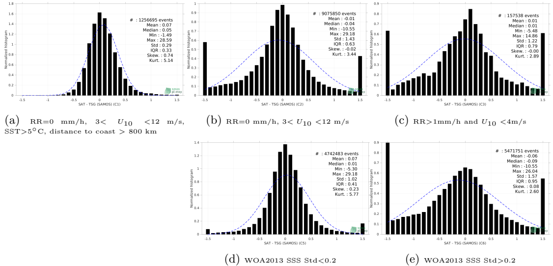
Figure 13: Normalized histogram of \Delta SSS (SMOS SSS L3 v2 - 9-Days (BEC) - TSG (SAMOS)) for 5 different subdatasets corresponding to: RR=0 mm/h, 3 < U_{10} < 12 m/s, SST >5^\circ\text{C} , distance to coast > 800 km (a), RR=0 mm/h, 3 < U_{10} < 12 m/s (b), RR >1 mm/h and U_{10} < 4 m/s (c), WOA2013 SSS Std <0.2 (d), WOA2013 SSS Std >0.2 (e).
