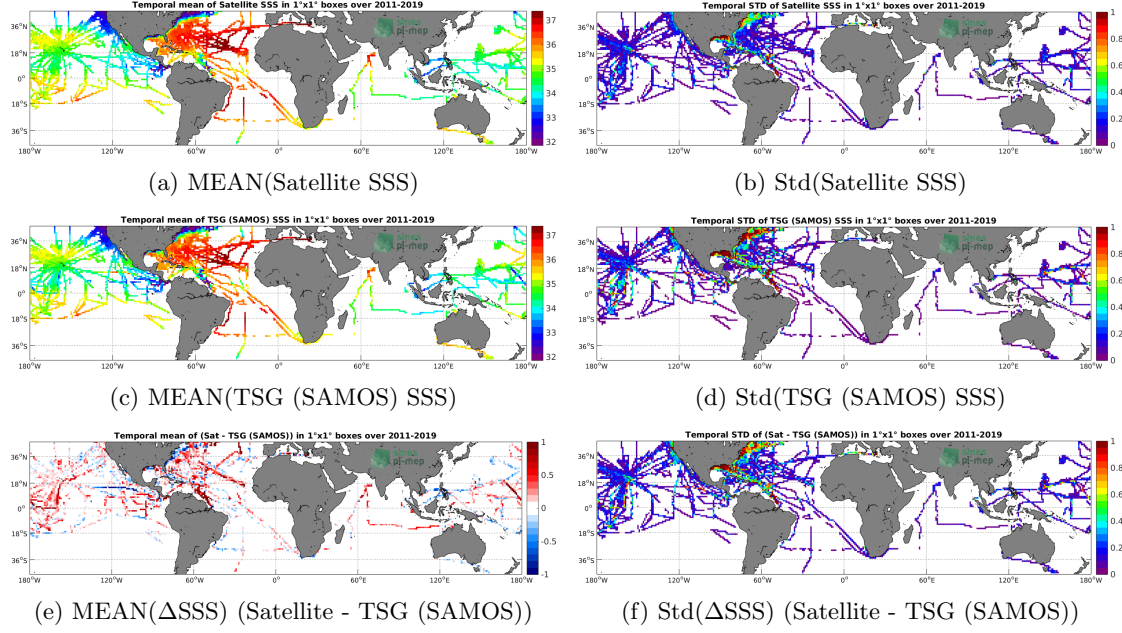
Figure 6: Temporal mean (left) and Std (right) of SSS from SMOS L3 v2 - 9-Days (BEC) (top), TSG (SAMOS) (middle), and of \Delta SSS (Satellite - TSG (SAMOS)). Only match-up pairs are used to generate these maps.
