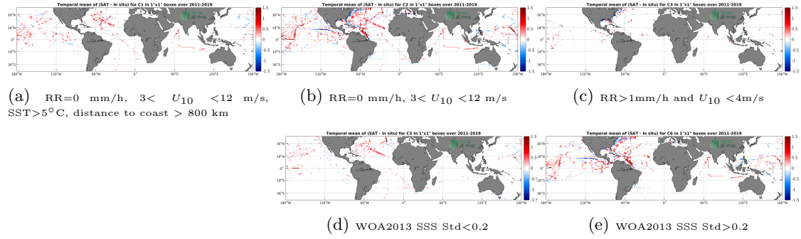
Figure 12: Temporal mean gridded over spatial boxes of size 1^\circ \times 1^\circ of \Delta SSS (SMOS L3 v2 - 9-Days (BEC) - TSG (SAMOS)) for 5 different subdatasets corresponding to: RR=0 mm/h, 3 < U_{10} < 12 m/s, SST > 5^\circ C , distance to coast > 800 km (a), RR=0 mm/h, 3 < U_{10} < 12 m/s (b), RR > 1 mm/h and U_{10} < 4 m/s (c), WOA2013 SSS Std < 0.2 (d), WOA2013 SSS Std > 0.2 (e).
