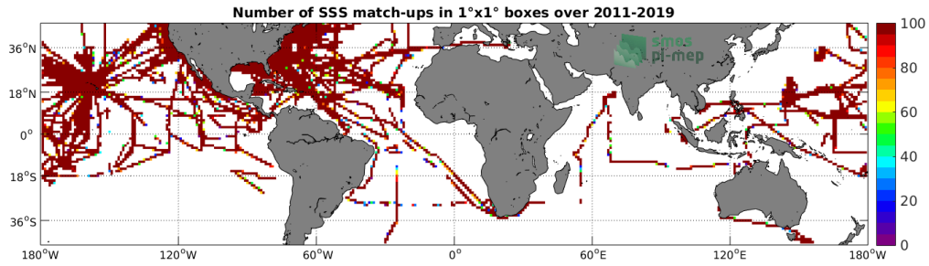
Figure 4: Number of SSS match-ups between TSG (SAMOS) SSS and the SMOS L3 v2 - 9-Days (BEC) SSS product for the Mid-Low Latitudes 45N-45S Pi-MEP region over 1°x1° boxes and for the full satellite product period.
