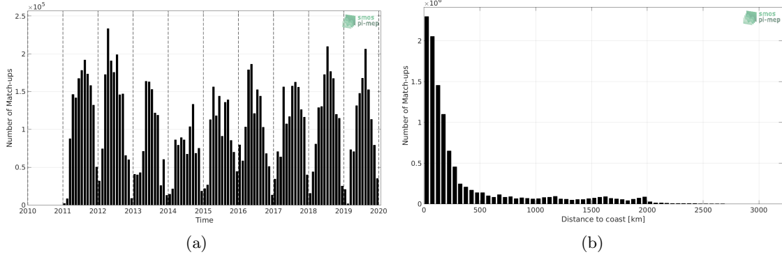
Figure 1: Number of match-ups between TSG (SAMOS) and SMOS L3 v2 - 9-Days (BEC) SSS as a function of time (a) and as function of the distance to coast (b) over the Mid-Low Latitudes 45N-45S Pi-MEP region and for the full satellite product period.
