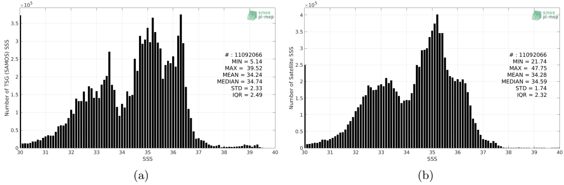
Figure 2: Histograms of SSS from TSG (SAMOS) (a) and SMOS L3 v2 - 9-Days (BEC) (b) considering all match-up pairs per bins of 0.1 over the Mid-Low Latitudes 45N-45S Pi-MEP region and for the full satellite product period.
