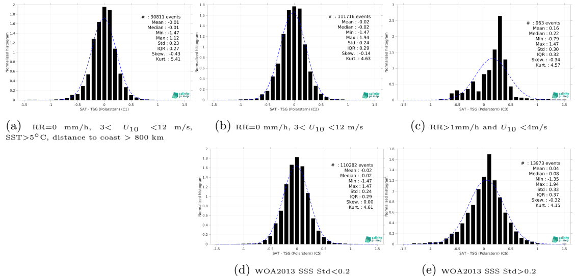
Figure 13: Normalized histogram of \Delta\text{SSS} (SMOS SSS L3 v2 - 9-Days (BEC) - TSG (Polarstern)) for 5 different subdatasets corresponding to: RR=0 mm/h, 3 < U_{10} < 12 m/s, SST >5^\circ\text{C} , distance to coast > 800 km (a), RR=0 mm/h, 3 < U_{10} < 12 m/s (b), RR >1 mm/h and U_{10} < 4 m/s (c), WOA2013 SSS Std <0.2 (d), WOA2013 SSS Std >0.2 (e).
