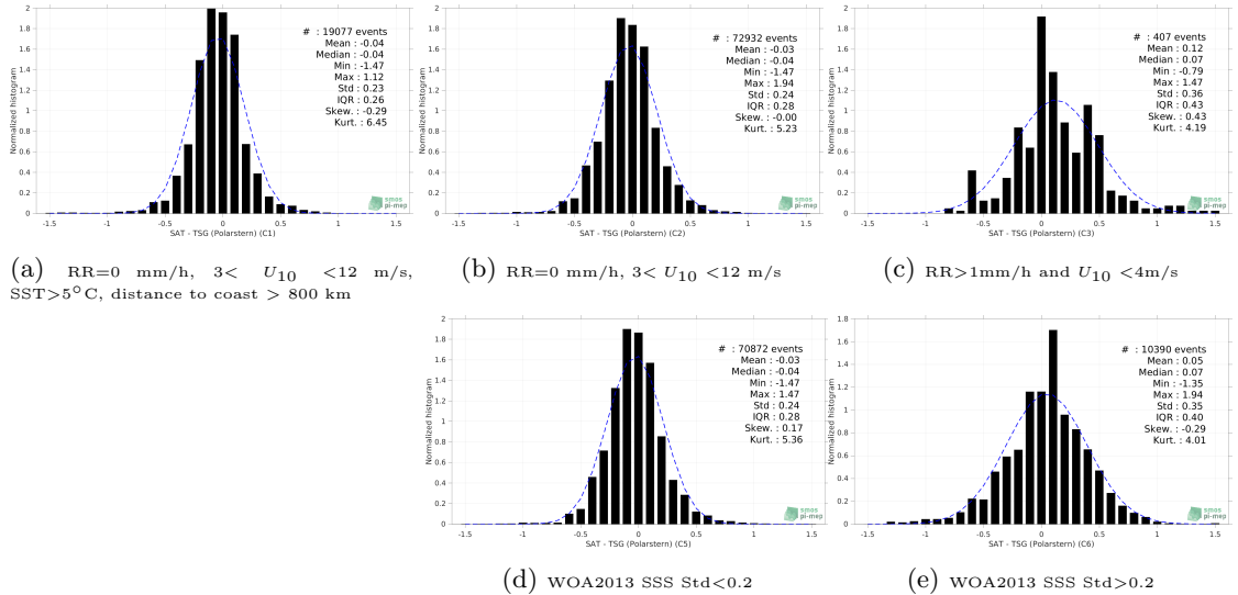
Figure 13: Normalized histogram of \Delta SSS (SMOS SSS L3 v2 - 9-Days (BEC) - TSG (Polarstern)) for 5 different subdatasets corresponding to: RR=0 mm/h, 3 < U_{10} < 12 m/s, SST >5^\circ\text{C} , distance to coast > 800 km (a), RR=0 mm/h, 3 < U_{10} < 12 m/s (b), RR >1 mm/h and U_{10} < 4 m/s (c), WOA2013 SSS Std <0.2 (d), WOA2013 SSS Std >0.2 (e).
