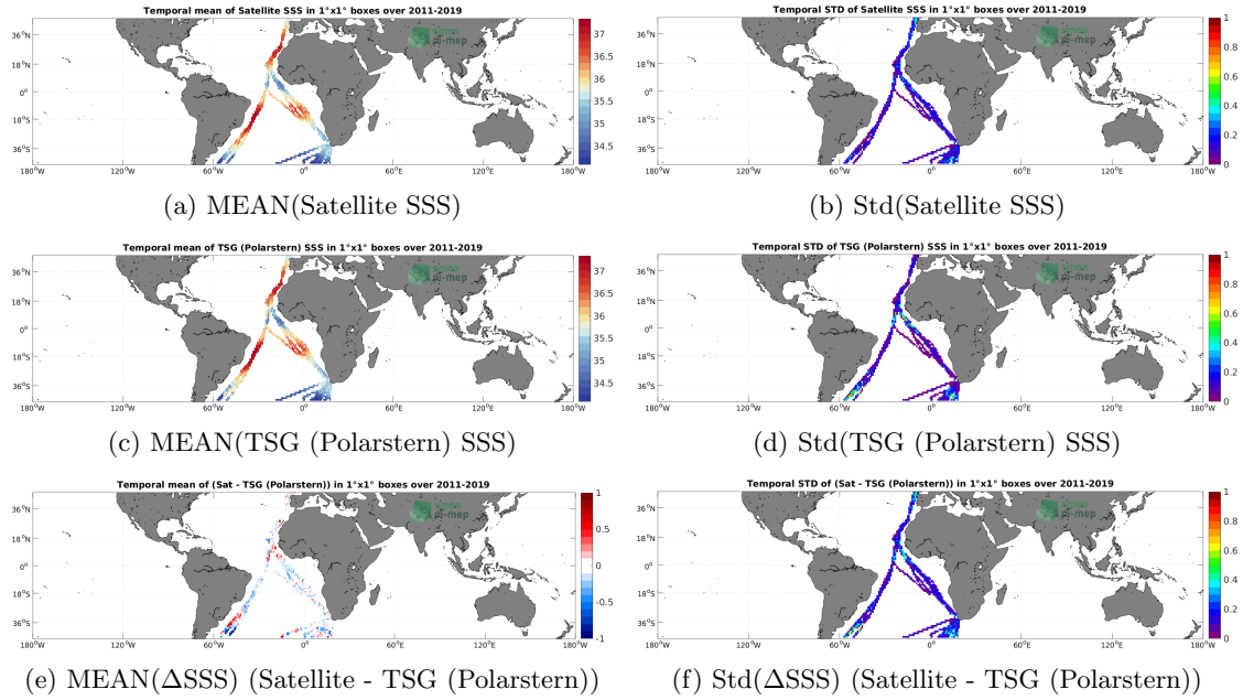
Figure 6: Temporal mean (left) and Std (right) of SSS from SMOS SSS L3 v2 - 9-Days (BEC) (top), TSG (Polarstern) (middle), and of \Delta SSS (Satellite - TSG (Polarstern)). Only match-up pairs are used to generate these maps.
