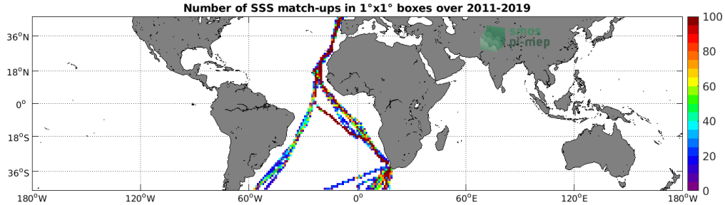
Figure 4: Number of SSS match-ups between TSG (Polarstern) SSS and the SMOS SSS L3 v2 - 9-Days (BEC) SSS product for the Mid-Low Latitudes 45N-45S Pi-MEP region over 1^\circ \times 1^\circ boxes and for the full satellite product period.
