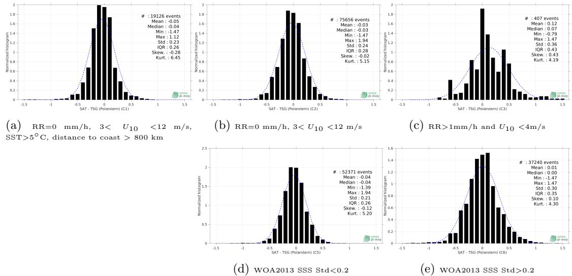
Figure 13: Normalized histogram of \Delta SSS (SMOS SSS L3 v2 - 9-Days (BEC) - TSG (Polarstern)) for 5 different subdatasets corresponding to: RR=0 mm/h, 3 < U_{10} < 12 m/s, SST > 5^\circ C , distance to coast > 800 km (a), RR=0 mm/h, 3 < U_{10} < 12 m/s (b), RR > 1 mm/h and U_{10} < 4 m/s (c), WOA2013 SSS Std < 0.2 (d), WOA2013 SSS Std > 0.2 (e).
