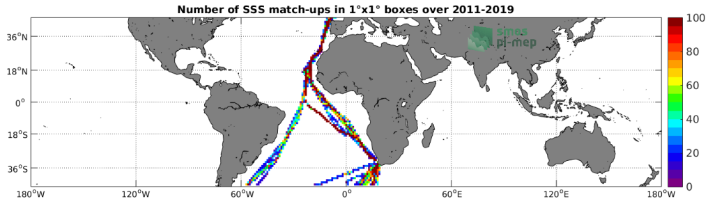
Figure 4: Number of SSS match-ups between TSG (Polarstern) SSS and the SMOS L3 v2 - 9-Days (BEC) SSS product for the Mid-Low Latitudes 45N-45S Pi-MEP region over 1^\circ \times 1^\circ boxes and for the full satellite product period.
