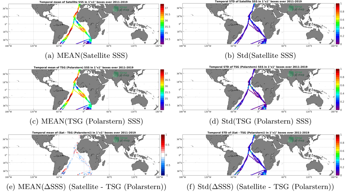
Figure 6: Temporal mean (left) and Std (right) of SSS from SMOS L3 v2 - 9-Days (BEC) (top), TSG (Polarstern) (middle), and of \Delta SSS (Satellite - TSG (Polarstern)). Only match-up pairs are used to generate these maps.
