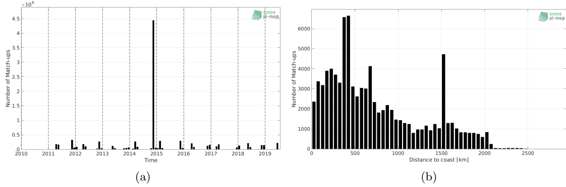
Figure 1: Number of match-ups between TSG (Polarstern) and SMOS L3 v2 - 9-Days (BEC) SSS as a function of time (a) and as function of the distance to coast (b) over the Mid-Low Latitudes 45N-45S Pi-MEP region and for the full satellite product period.
