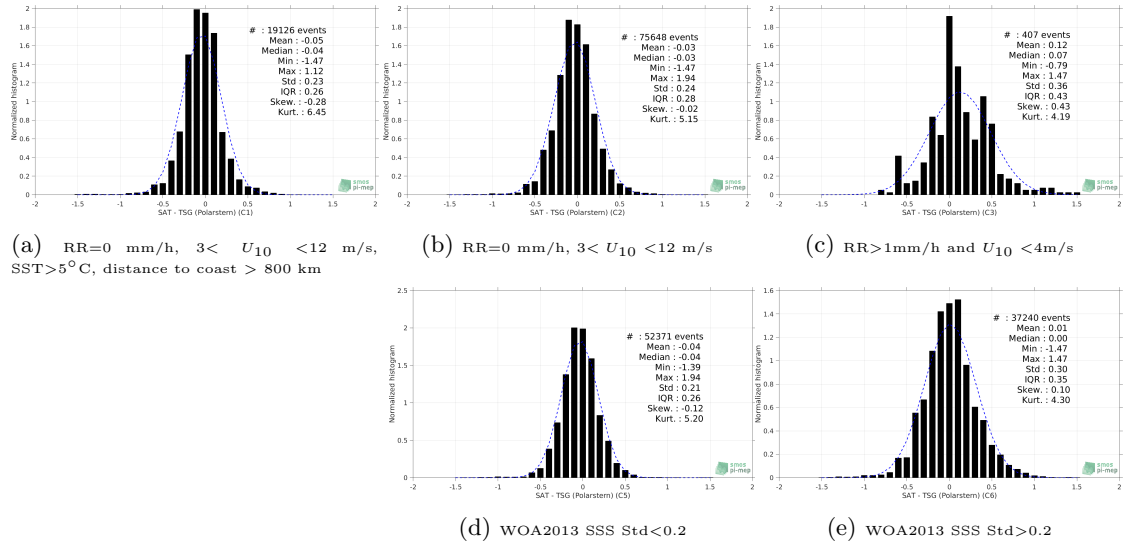
Figure 13: Normalized histogram of \Delta SSS (SMOS L3 v2 - 9-Days (BEC) - TSG (Polarstern)) for 5 different subdatasets corresponding to: RR=0 mm/h, 3 < U_{10} < 12 m/s, SST > 5^\circ C , distance to coast > 800 km (a), RR=0 mm/h, 3 < U_{10} < 12 m/s (b), RR > 1 mm/h and U_{10} < 4 m/s (c), WOA2013 SSS Std < 0.2 (d), WOA2013 SSS Std > 0.2 (e).
