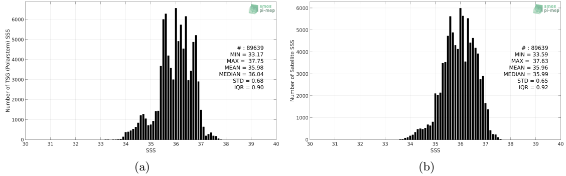
Figure 2: Histograms of SSS from TSG (Polarstern) (a) and SMOS L3 v2 - 9-Days (BEC) (b) considering all match-up pairs per bins of 0.1 over the Mid-Low Latitudes 45N-45S Pi-MEP region and for the full satellite product period.
