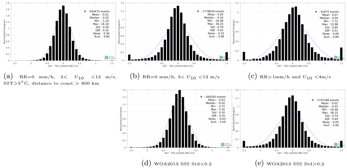
Figure 13: Normalized histogram of \Delta SSS (SMOS SSS L3 v2 - 9-Days (BEC) - TSG (LEGOS-DM)) for 5 different subdatasets corresponding to: RR=0 mm/h, 3 < U_{10} < 12 m/s, SST > 5^\circ C , distance to coast > 800 km (a), RR=0 mm/h, 3 < U_{10} < 12 m/s (b), RR > 1 mm/h and U_{10} < 4 m/s (c), WOA2013 SSS Std < 0.2 (d), WOA2013 SSS Std > 0.2 (e).
