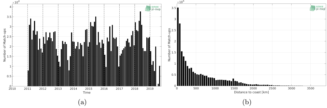
Figure 1: Number of match-ups between TSG (LEGOS-DM) and SMOS L3 v2 - 9-Days (BEC) SSS as a function of time (a) and as function of the distance to coast (b) over the Mid-Low Latitudes 45N-45S Pi-MEP region and for the full satellite product period.
