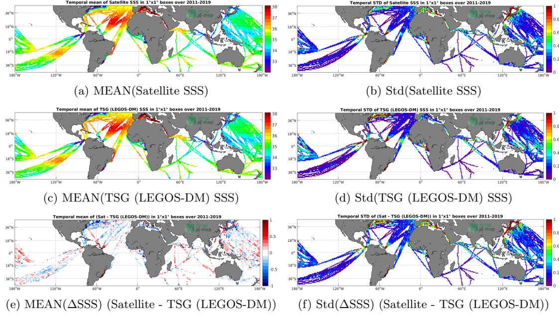
Figure 6: Temporal mean (left) and Std (right) of SSS from SMOS L3 v2 - 9-Days (BEC) (top), TSG (LEGOS-DM) (middle), and of \Delta SSS (Satellite - TSG (LEGOS-DM)). Only match-up pairs are used to generate these maps.
