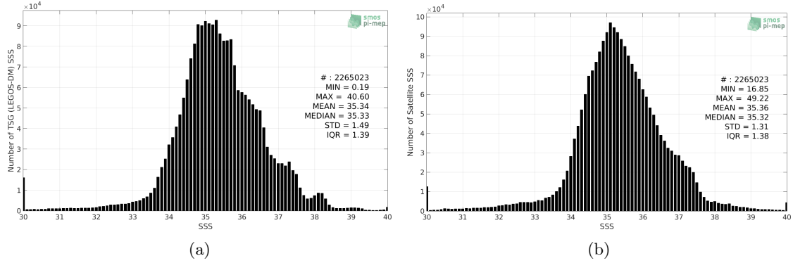
Figure 2: Histograms of SSS from TSG (LEGOS-DM) (a) and SMOS L3 v2 - 9-Days (BEC) (b) considering all match-up pairs per bins of 0.1 over the Mid-Low Latitudes 45N-45S Pi-MEP region and for the full satellite product period.
