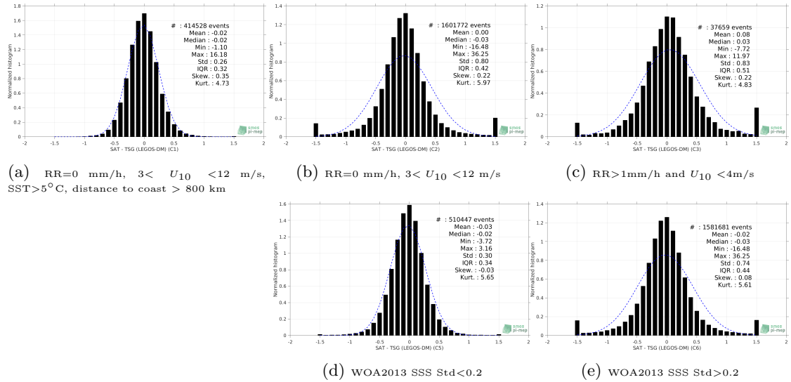
Figure 13: Normalized histogram of \Delta SSS (SMOS L3 v2 - 9-Days (BEC) - TSG (LEGOS-DM)) for 5 different subdatasets corresponding to: RR=0 mm/h, 3 < U_{10} < 12 m/s, SST > 5^\circ C , distance to coast > 800 km (a), RR=0 mm/h, 3 < U_{10} < 12 m/s (b), RR > 1 mm/h and U_{10} < 4 m/s (c), WOA2013 SSS Std < 0.2 (d), WOA2013 SSS Std > 0.2 (e).
