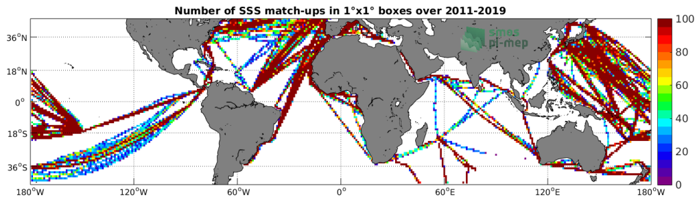
Figure 4: Number of SSS match-ups between TSG (LEGOS-DM) SSS and the SMOS L3 v2 - 9-Days (BEC) SSS product for the Mid-Low Latitudes 45N-45S Pi-MEP region over 1^\circ \times 1^\circ boxes and for the full satellite product period.
