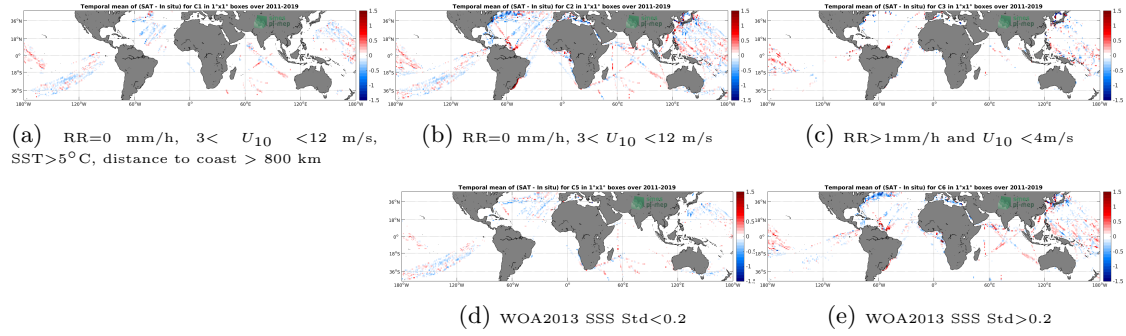
Figure 12: Temporal mean gridded over spatial boxes of size 1^\circ \times 1^\circ of \Delta SSS (SMOS L3 v2 - 9-Days (BEC) - TSG (LEGOS-DM)) for 5 different subdatasets corresponding to: RR=0 mm/h, 3 < U_{10} < 12 m/s, SST > 5^\circ C , distance to coast > 800 km (a), RR=0 mm/h, 3 < U_{10} < 12 m/s (b), RR > 1 mm/h and U_{10} < 4 m/s (c), WOA2013 SSS Std < 0.2 (d), WOA2013 SSS Std > 0.2 (e).
