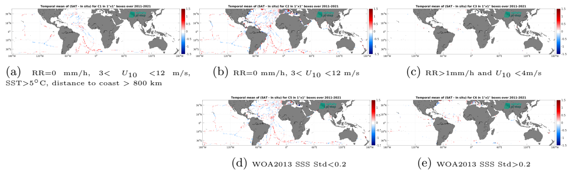
Figure 12: Temporal mean gridded over spatial boxes of size 1^\circ \times 1^\circ of \Delta\text{SSS} (SMOS SSS L3 v2 - 9-Days (BEC) - TSG (GOSUD-Sailing-ship)) for 5 different subdatasets corresponding to: RR=0 mm/h, 3 < U_{10} < 12 m/s, SST > 5^\circ\text{C} , distance to coast > 800 km (a), RR=0 mm/h, 3 < U_{10} < 12 m/s (b), RR > 1\text{mm/h} and U_{10} < 4\text{m/s} (c), WOA2013 SSS Std < 0.2 (d), WOA2013 SSS Std > 0.2 (e).
