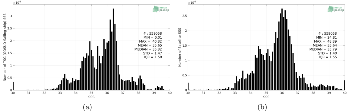
Figure 2: Histograms of SSS from TSG (GOSUD-Sailing-ship) (a) and SMOS SSS L3 v2 - 9-Days (BEC) (b) considering all match-up pairs per bins of 0.1 over the Mid-Low Latitudes 45N-45S Pi-MEP region and for the full satellite product period.
