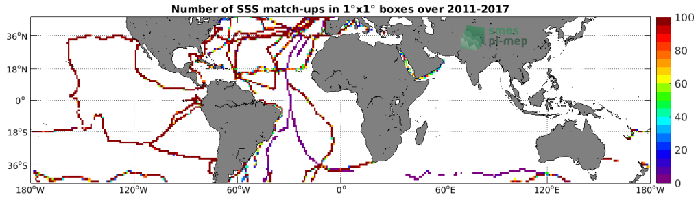
Figure 4: Number of SSS match-ups between TSG (GOSUD-Sailing-ship) SSS and the SMOS SSS L3 v2 - 9-Days (BEC) SSS product for the Mid-Low Latitudes 45N-45S Pi-MEP region over 1^\circ \times 1^\circ boxes and for the full satellite product period.
