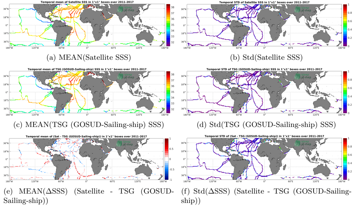
Figure 6: Temporal mean (left) and Std (right) of SSS from SMOS SSS L3 v2 - 9-Days (BEC) (top), TSG (GOSUD-Sailing-ship) (middle), and of \Delta SSS (Satellite - TSG (GOSUD-Sailing-ship)). Only match-up pairs are used to generate these maps.
