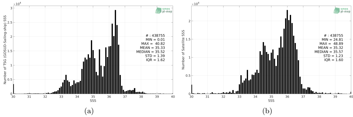
Figure 2: Histograms of SSS from TSG (GOSUD-Sailing-ship) (a) and SMOS SSS L3 v2 - 9-Days (BEC) (b) considering all match-up pairs per bins of 0.1 over the Mid-Low Latitudes 45N-45S Pi-MEP region and for the full satellite product period.
