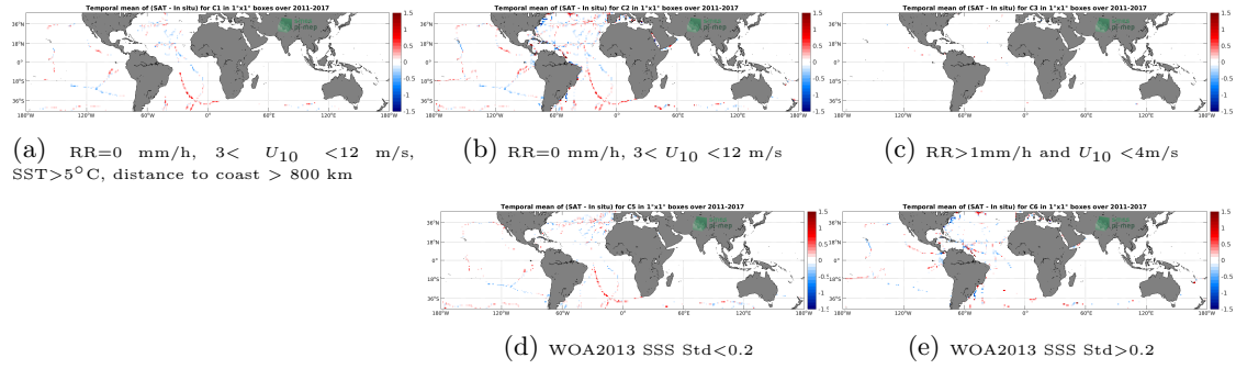
Figure 12: Temporal mean gridded over spatial boxes of size 1^\circ \times 1^\circ of \Delta SSS (SMOS SSS L3 v2 - 9-Days (BEC) - TSG (GOSUD-Sailing-ship)) for 5 different subdatasets corresponding to: RR=0 mm/h, 3 < U_{10} < 12 m/s, SST > 5^\circ C , distance to coast > 800 km (a), RR=0 mm/h, 3 < U_{10} < 12 m/s (b), RR > 1 mm/h and U_{10} < 4 m/s (c), WOA2013 SSS Std < 0.2 (d), WOA2013 SSS Std > 0.2 (e).
