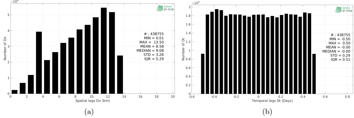
Figure 5: Histograms of the spatial (a) and temporal (b) lags between the time of the TSG (GOSUD-Sailing-ship) measurements and the date of the corresponding SMOS SSS L3 v2 - 9-Days (BEC) SSS product.
