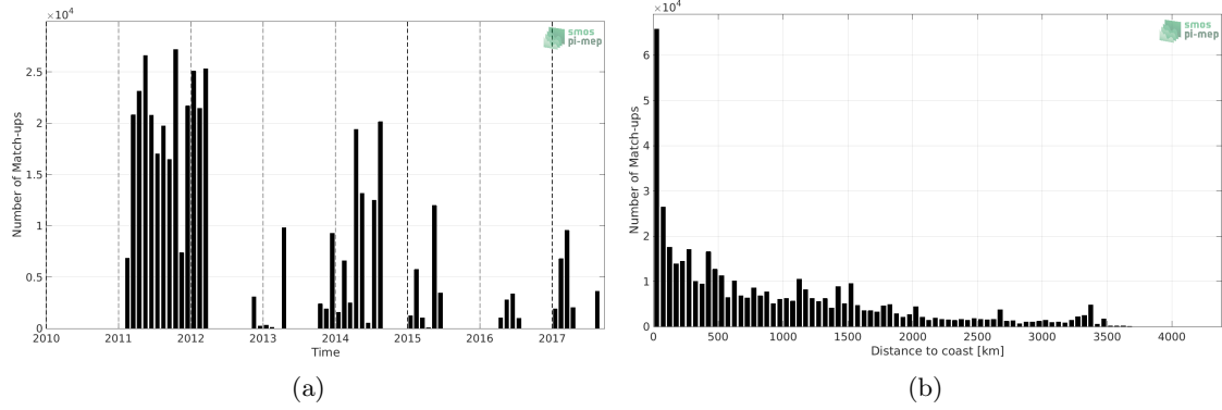
Figure 1: Number of match-ups between TSG (GOSUD-Sailing-ship) and SMOS SSS L3 v2 - 9-Days (BEC) SSS as a function of time (a) and as function of the distance to coast (b) over the Mid-Low Latitudes 45N-45S Pi-MEP region and for the full satellite product period.
