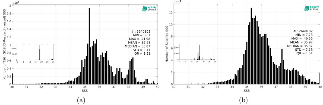
Figure 3: Histograms of SSS from TSG (GOSUD-Research-vessel) (a) and SMOS SSS L3 v2 - 9-Days (BEC) (b) considering all match-up pairs per bins of 0.1 over the Mid-Low Latitudes 45N-45S Pi-MEP region and for the full satellite product period.
