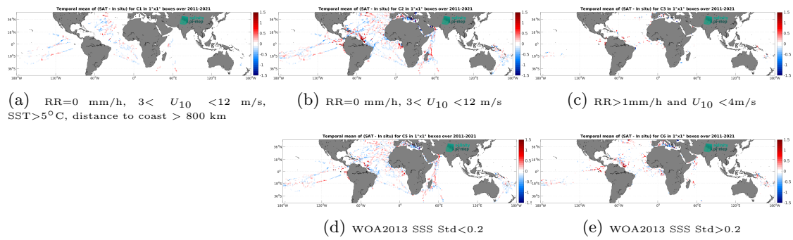
Figure 14: Temporal mean gridded over spatial boxes of size 1^\circ \times 1^\circ of \Delta\text{SSS} (SMOS SSS L3 v2 - 9-Days (BEC) - TSG (GOSUD-Research-vessel)) for 5 different subdatasets corresponding to: RR=0 mm/h, 3 < U_{10} < 12 m/s, SST > 5°C, distance to coast > 800 km (a), RR=0 mm/h, 3 < U_{10} < 12 m/s (b), RR > 1mm/h and U_{10} < 4 m/s (c), WOA2013 SSS Std < 0.2 (d), WOA2013 SSS Std > 0.2 (e).
