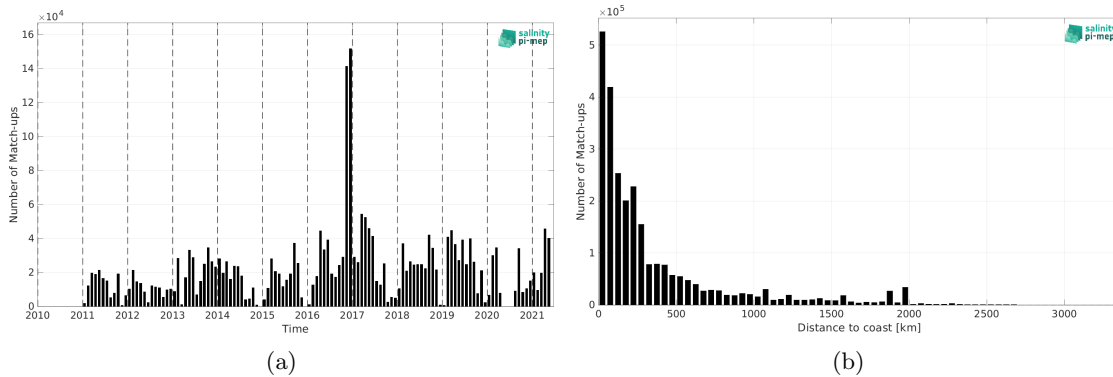
Figure 2: Number of match-ups between TSG (GOSUD-Research-vessel) and SMOS SSS L3 v2 - 9-Days (BEC) SSS as a function of time (a) and as function of the distance to coast (b) over the Mid-Low Latitudes 45N-45S Pi-MEP region and for the full satellite product period.
