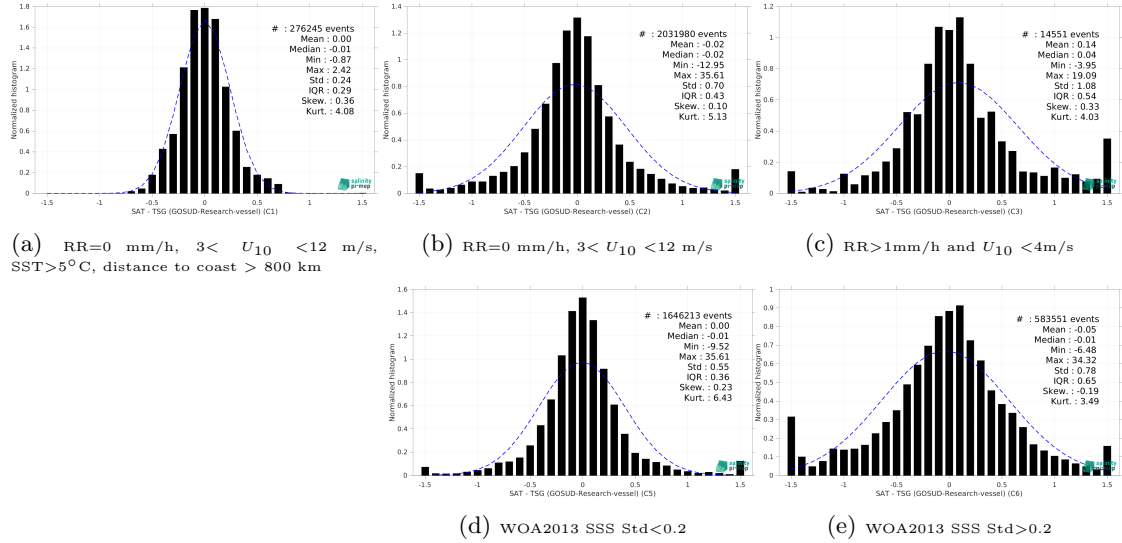
Figure 15: Normalized histogram of \Delta\text{SSS} (SMOS SSS L3 v2 - 9-Days (BEC) - TSG (GOSUD-Research-vessel)) for 5 different subdatasets corresponding to: RR=0 mm/h, 3 < U_{10} < 12 m/s, SST > 5^\circ\text{C} , distance to coast > 800 km (a), RR=0 mm/h, 3 < U_{10} < 12 m/s (b), RR > 1 mm/h and U_{10} < 4 m/s (c), WOA2013 SSS Std < 0.2 (d), WOA2013 SSS Std > 0.2 (e).
