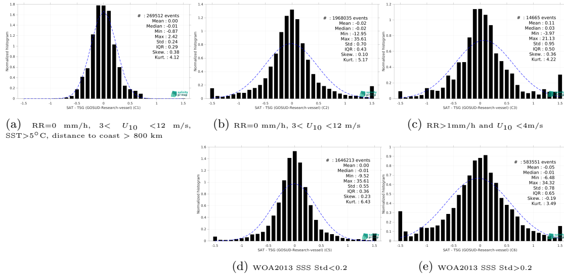
Figure 15: Normalized histogram of \Delta\text{SSS} (SMOS SSS L3 v2 - 9-Days (BEC) - TSG (GOSUD-Research-vessel)) for 5 different subdatasets corresponding to: RR=0 mm/h, 3 < U_{10} < 12 m/s, SST > 5^\circ\text{C} , distance to coast > 800 km (a), RR=0 mm/h, 3 < U_{10} < 12 m/s (b), RR > 1 mm/h and U_{10} < 4 m/s (c), WOA2013 SSS Std < 0.2 (d), WOA2013 SSS Std > 0.2 (e).
