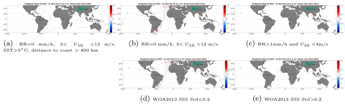
Figure 14: Temporal mean gridded over spatial boxes of size 1^\circ \times 1^\circ of \Delta SSS (SMOS SSS L3 v2 - 9-Days (BEC) - TSG (CSIC-UTM)) for 5 different subdatasets corresponding to: RR=0 mm/h, 3 < U_{10} < 12 m/s, SST > 5°C, distance to coast > 800 km (a), RR=0 mm/h, 3 < U_{10} < 12 m/s (b), RR > 1mm/h and U_{10} < 4 m/s (c), WOA2013 SSS Std < 0.2 (d), WOA2013 SSS Std > 0.2 (e).
