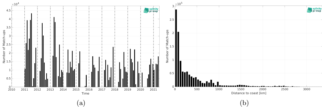
Figure 2: Number of match-ups between TSG (CSIC-UTM) and SMOS SSS L3 v2 - 9-Days (BEC) SSS as a function of time (a) and as function of the distance to coast (b) over the Mid-Low Latitudes 45N-45S Pi-MEP region and for the full satellite product period.
