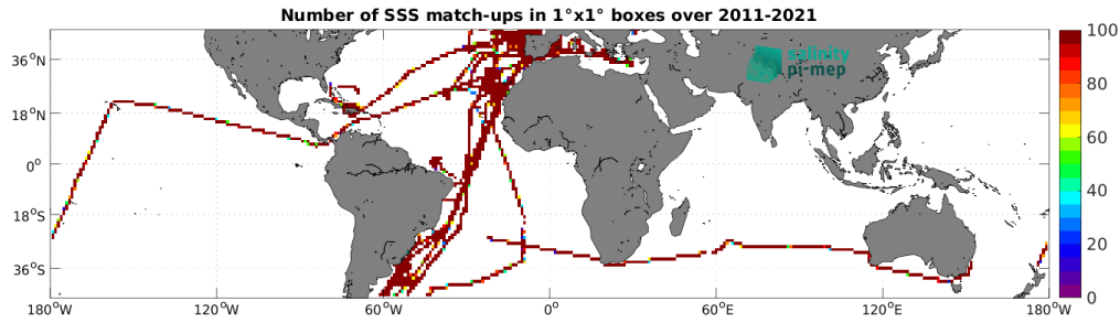
Figure 5: Number of SSS match-ups between TSG (CSIC-UTM) SSS and the SMOS SSS L3 v2 - 9-Days (BEC) SSS product for the Mid-Low Latitudes 45N-45S Pi-MEP region over 1^\circ \times 1^\circ boxes and for the full satellite product period.
