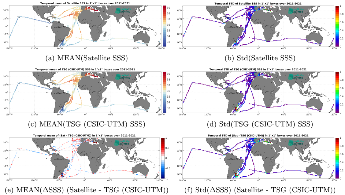
Figure 7: Temporal mean (left) and Std (right) of SSS from SMOS SSS L3 v2 - 9-Days (BEC) (top), TSG (CSIC-UTM) (middle), and of \Delta SSS (Satellite - TSG (CSIC-UTM)). Only match-up pairs are used to generate these maps.
