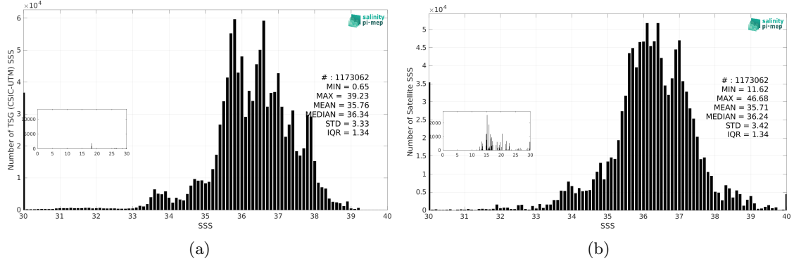
Figure 3: Histograms of SSS from TSG (CSIC-UTM) (a) and SMOS SSS L3 v2 - 9-Days (BEC) (b) considering all match-up pairs per bins of 0.1 over the Mid-Low Latitudes 45N-45S Pi-MEP region and for the full satellite product period.
