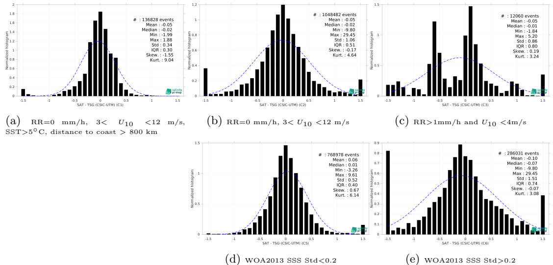
Figure 13: Normalized histogram of \Delta\text{SSS} (SMOS SSS L3 v2 - 9-Days (BEC) - TSG (CSIC-UTM)) for 5 different subdatasets corresponding to: RR=0 mm/h, 3 < U_{10} < 12 m/s, SST >5^\circ\text{C} , distance to coast > 800 km (a), RR=0 mm/h, 3 < U_{10} < 12 m/s (b), RR >1 mm/h and U_{10} < 4 m/s (c), WOA2013 SSS Std <0.2 (d), WOA2013 SSS Std >0.2 (e).
