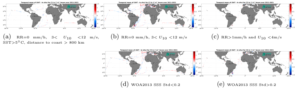
Figure 12: Temporal mean gridded over spatial boxes of size 1^\circ \times 1^\circ of \Delta\text{SSS} (SMOS SSS L3 v2 - 9-Days (BEC) - TSG (CSIC-UTM)) for 5 different subdatasets corresponding to: RR=0 mm/h, 3 < U_{10} < 12 m/s, SST >5^\circ\text{C} , distance to coast > 800 km (a), RR=0 mm/h, 3 < U_{10} < 12 m/s (b), RR >1 mm/h and U_{10} < 4 m/s (c), WOA2013 SSS Std <0.2 (d), WOA2013 SSS Std >0.2 (e).
