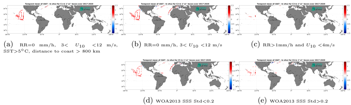
Figure 14: Temporal mean gridded over spatial boxes of size 1^\circ \times 1^\circ of \Delta\text{SSS} (SMOS SSS L3 v2 - 9-Days (BEC) - Saildrone) for 5 different subdatasets corresponding to:RR=0 mm/h, 3 < U_{10} < 12 m/s, SST>5°C, distance to coast > 800 km (a), RR=0 mm/h, 3 < U_{10} < 12 m/s (b), RR>1mm/h and U_{10} < 4 m/s (c), WOA2013 SSS Std<0.2 (d), WOA2013 SSS Std>0.2 (e).
