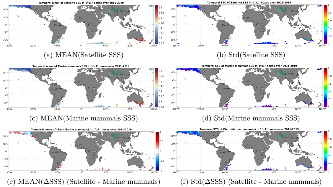
Figure 6: Temporal mean (left) and Std (right) of SSS from SMOS SSS L3 v2 - 9-Days (BEC) (top), Marine mammals (middle), and of \Delta SSS (Satellite - Marine mammals). Only match-up pairs are used to generate these maps.
