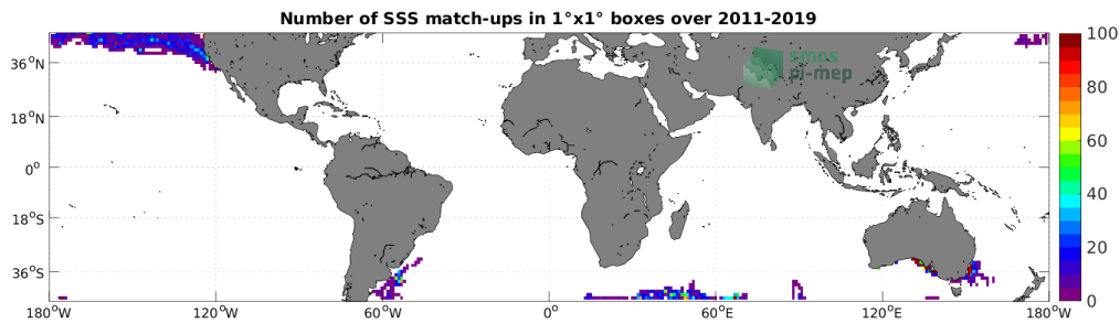
Figure 4: Number of SSS match-ups between Marine mammals SSS and the SMOS SSS L3 v2 - 9-Days (BEC) SSS product for the Mid-Low Latitudes 45N-45S Pi-MEP region over 1^\circ \times 1^\circ boxes and for the full satellite product period.
