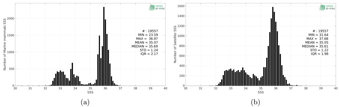
Figure 2: Histograms of SSS from Marine mammals (a) and SMOS SSS L3 v2 - 9-Days (BEC) (b) considering all match-up pairs per bins of 0.1 over the Mid-Low Latitudes 45N-45S Pi-MEP region and for the full satellite product period.
