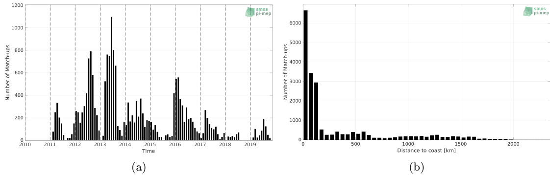
Figure 1: Number of match-ups between Marine mammals and SMOS SSS L3 v2 - 9-Days (BEC) SSS as a function of time (a) and as function of the distance to coast (b) over the Mid-Low Latitudes 45N-45S Pi-MEP region and for the full satellite product period.
