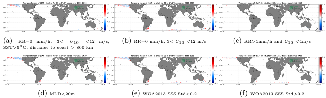
Figure 12: Temporal mean gridded over spatial boxes of size 1^\circ \times 1^\circ of \Delta SSS (SMOS SSS L3 v2 - 9-Days (BEC) - Marine mammals) for 6 different subdatasets corresponding to:RR=0 mm/h, 3 < U_{10} < 12 m/s, SST >5^\circ\text{C} , distance to coast > 800 km (a), RR=0 mm/h, 3 < U_{10} < 12 m/s (b), RR >1 mm/h and U_{10} < 4 m/s (c),MLD <20 m (d),WOA2013 SSS Std <0.2 (e),WOA2013 SSS Std >0.2 (f).
