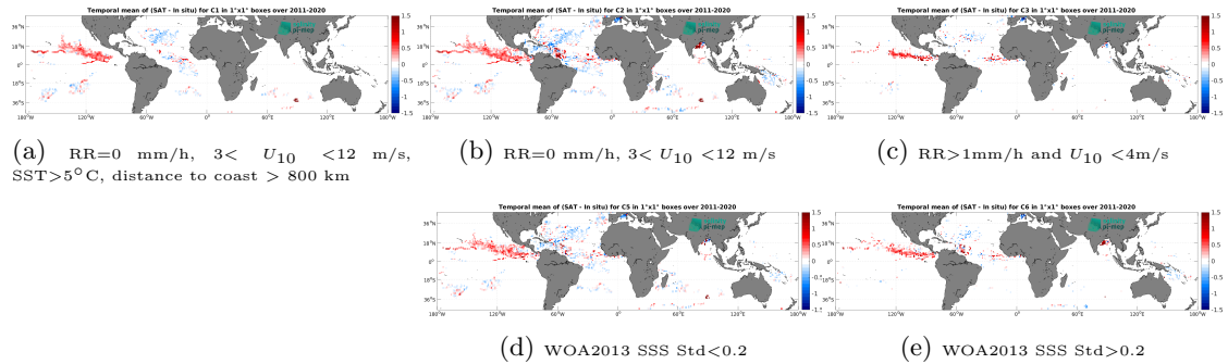
Figure 13: Temporal mean gridded over spatial boxes of size 1^\circ \times 1^\circ of \Delta SSS (SMOS SSS L3 v2 - 9-Days (BEC) - Surface drifters) for 5 different subdatasets corresponding to: RR=0 mm/h, 3 < U_{10} < 12 m/s, SST>5°C, distance to coast > 800 km (a), RR=0 mm/h, 3 < U_{10} < 12 m/s (b), RR>1mm/h and U_{10} < 4 m/s (c), WOA2013 SSS Std<0.2 (d), WOA2013 SSS Std>0.2 (e).
