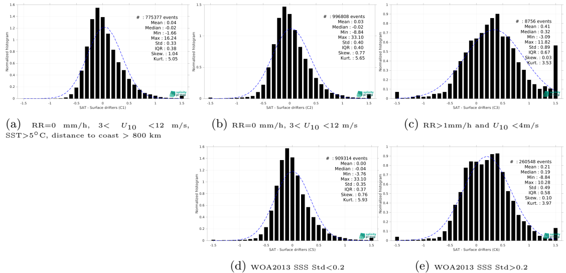
Figure 14: Normalized histogram of \Delta SSS (SMOS SSS L3 v2 - 9-Days (BEC) - Surface drifters) for 5 different subdatasets corresponding to: RR=0 mm/h, 3 < U_{10} < 12 m/s, SST>5°C, distance to coast > 800 km (a), RR=0 mm/h, 3 < U_{10} < 12 m/s (b), RR>1mm/h and U_{10} < 4 m/s (c), WOA2013 SSS Std<0.2 (d), WOA2013 SSS Std>0.2 (e).
