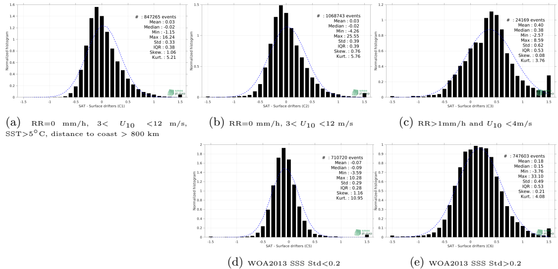
Figure 12: Normalized histogram of \Delta SSS (SMOS SSS L3 v2 - 9-Days (BEC) - Surface drifters) for 5 different subdatasets corresponding to: RR=0 mm/h, 3 < U_{10} < 12 m/s, SST >5^\circ\text{C} , distance to coast > 800 km (a), RR=0 mm/h, 3 < U_{10} < 12 m/s (b), RR >1 mm/h and U_{10} < 4 m/s (c), WOA2013 SSS Std <0.2 (d), WOA2013 SSS Std >0.2 (e).
