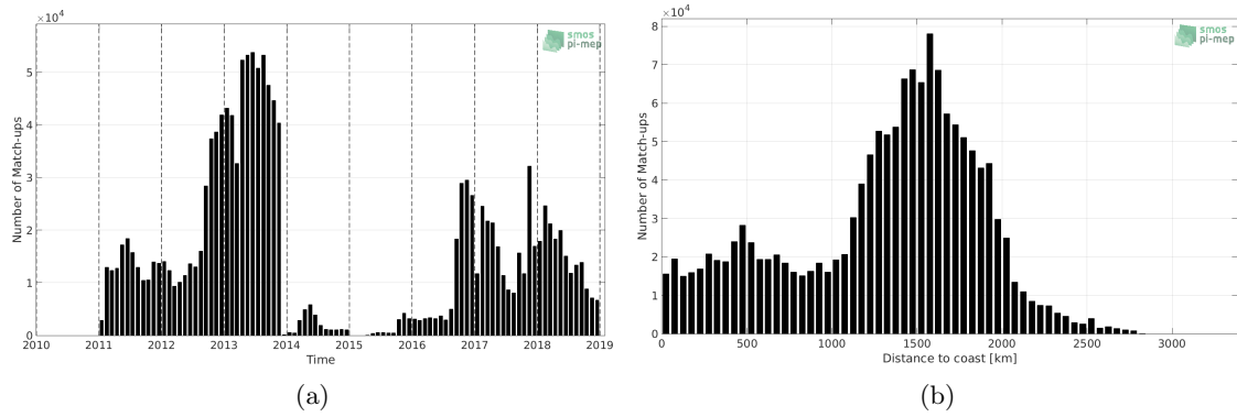
Figure 1: Number of match-ups between Surface drifters and SMOS L3 v2 - 9-Days (BEC) SSS as a function of time (a) and as function of the distance to coast (b) over the Mid-Low Latitudes 45N-45S Pi-MEP region and for the full satellite product period.
