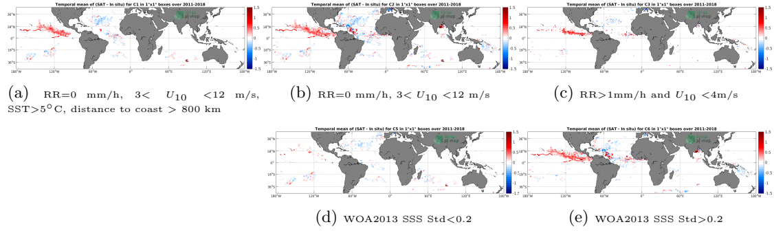
Figure 11: Temporal mean gridded over spatial boxes of size 1^\circ \times 1^\circ of \Delta SSS (SMOS L3 v2 - 9-Days (BEC) - Surface drifters) for 5 different subdatasets corresponding to: RR=0 mm/h, 3 < U_{10} < 12 m/s, SST > 5^\circ C , distance to coast > 800 km (a), RR=0 mm/h, 3 < U_{10} < 12 m/s (b), RR > 1 mm/h and U_{10} < 4 m/s (c), WOA2013 SSS Std < 0.2 (d), WOA2013 SSS Std > 0.2 (e).
