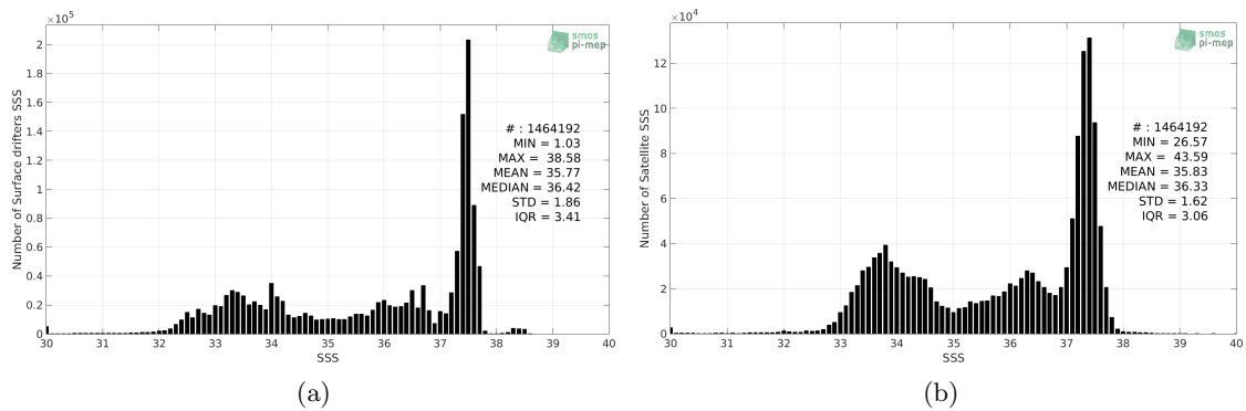
Figure 2: Histograms of SSS from Surface drifters (a) and SMOS L3 v2 - 9-Days (BEC) (b) considering all match-up pairs per bins of 0.1 over the Mid-Low Latitudes 45N-45S Pi-MEP region and for the full satellite product period.
