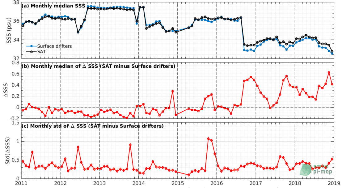
Figure 6: Time series of the monthly median SSS (top), median of \Delta\text{SSS} (Satellite - Surface drifters) and Std of \Delta\text{SSS} (Satellite - Surface drifters) over the Mid-Low Latitudes 45N-45S Pi-MEP region considering all match-ups collected by the Pi-MEP.
