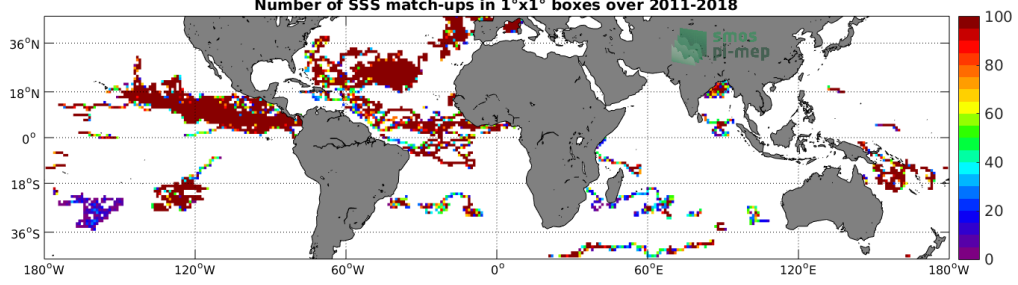
Figure 3: Number of SSS match-ups between Surface drifters SSS and the SMOS L3 v2 - 9-Days (BEC) SSS product for the Mid-Low Latitudes 45N-45S Pi-MEP region over 1°x1° boxes and for the full satellite product period.
