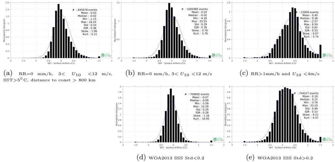
Figure 12: Normalized histogram of \Delta SSS (SMOS L3 v2 - 9-Days (BEC) - Surface drifters) for 5 different subdatasets corresponding to: RR=0 mm/h, 3 < U_{10} < 12 m/s, SST > 5^\circ C , distance to coast > 800 km (a), RR=0 mm/h, 3 < U_{10} < 12 m/s (b), RR > 1 mm/h and U_{10} < 4 m/s (c), WOA2013 SSS Std < 0.2 (d), WOA2013 SSS Std > 0.2 (e).
