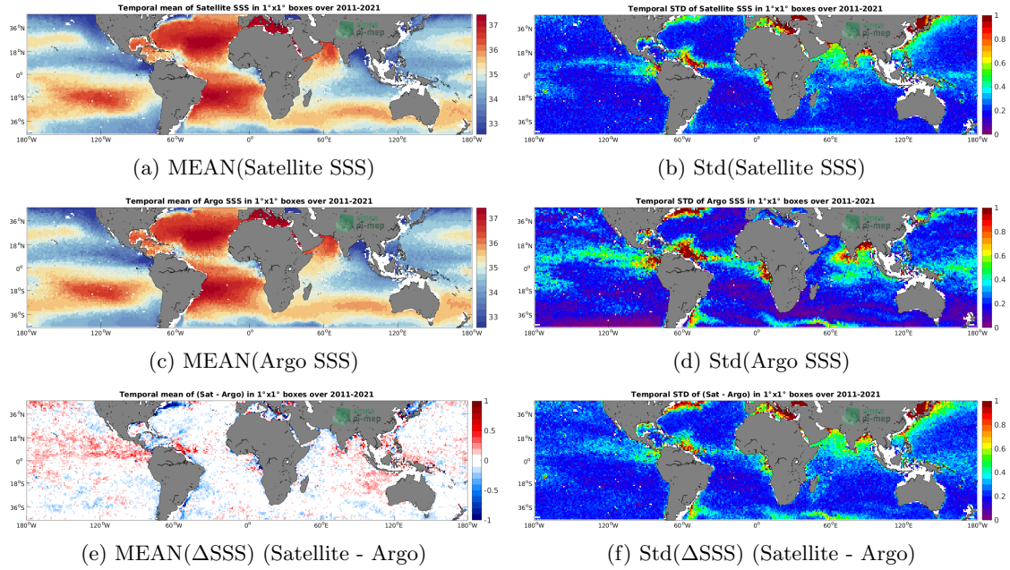
Figure 6: Temporal mean (left) and Std (right) of SSS from SMOS SSS L3 v2 - 9-Days (BEC) (top), Argo (middle), and of \Delta SSS (Satellite - Argo). Only match-up pairs are used to generate these maps.
