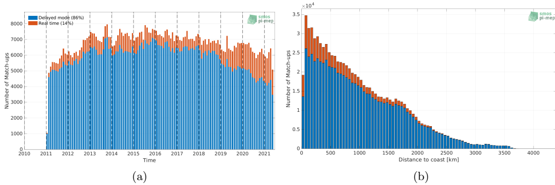
Figure 1: Number of match-ups between Argo and SMOS SSS L3 v2 - 9-Days (BEC) SSS as a function of time (a) and as function of the distance to coast (b) over the Mid-Low Latitudes 45N-45S Pi-MEP region and for the full satellite product period.
