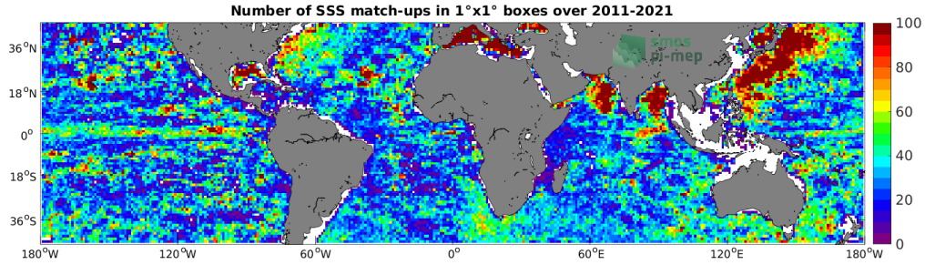
Figure 4: Number of SSS match-ups between Argo SSS and the SMOS SSS L3 v2 - 9-Days (BEC) SSS product for the Mid-Low Latitudes 45N-45S Pi-MEP region over 1^\circ \times 1^\circ boxes and for the full satellite product period.
