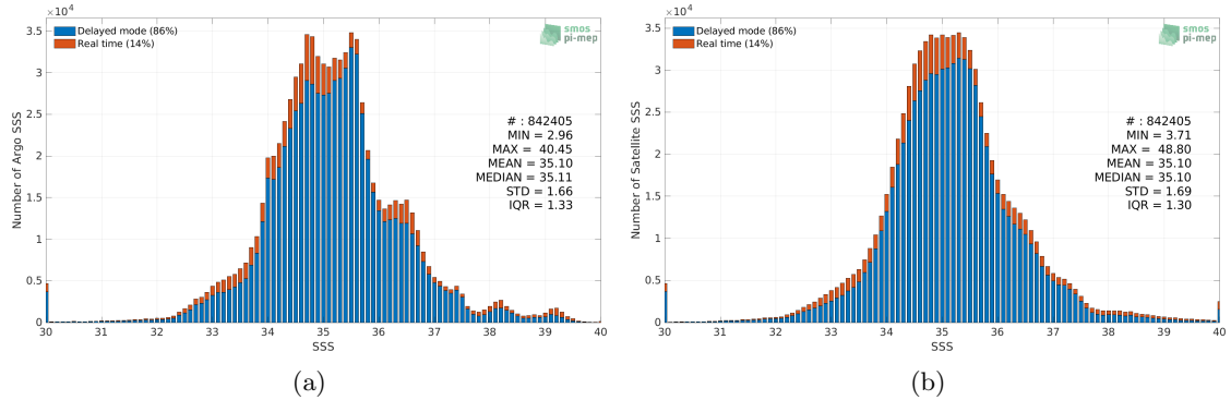
Figure 2: Histograms of SSS from Argo (a) and SMOS SSS L3 v2 - 9-Days (BEC) (b) considering all match-up pairs per bins of 0.1 over the Mid-Low Latitudes 45N-45S Pi-MEP region and for the full satellite product period.
