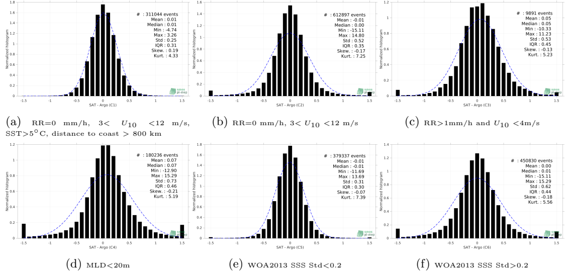
Figure 13: Normalized histogram of \Delta SSS (SMOS SSS L3 v2 - 9-Days (BEC) - Argo) for 6 different subdatasets corresponding to: RR=0 mm/h, 3 < U_{10} < 12 m/s, SST > 5°C, distance to coast > 800 km (a), RR=0 mm/h, 3 < U_{10} < 12 m/s (b), RR > 1mm/h and U_{10} < 4 m/s (c), MLD < 20m (d), WOA2013 SSS Std < 0.2 (e), WOA2013 SSS Std > 0.2 (f).
