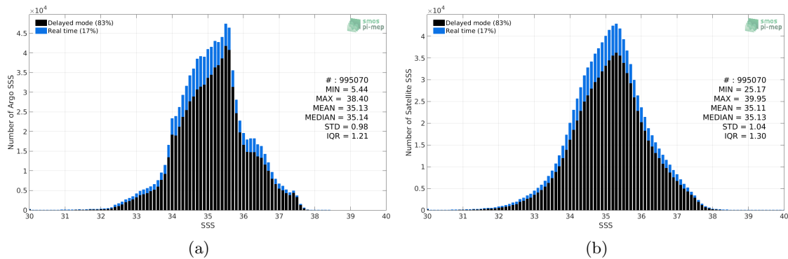
Figure 2: Histograms of SSS from Argo (a) and SMOS SSS L2-AVERAGED v700 (ESA) (b) considering all match-up pairs per bins of 0.1 over the Mid-Low Latitudes 45N-45S Pi-MEP region and for the full satellite product period.
