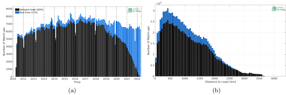
Figure 1: Number of match-ups between Argo and SMOS SSS L2-AVERAGED v700 (ESA) SSS as a function of time (a) and as function of the distance to coast (b) over the Mid-Low Latitudes 45N-45S Pi-MEP region and for the full satellite product period.
