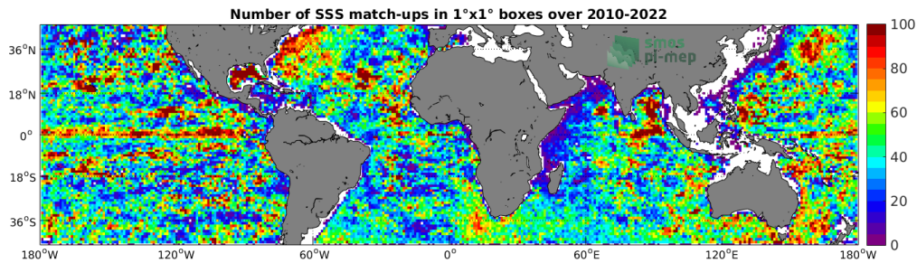
Figure 4: Number of SSS match-ups between Argo SSS and the SMOS SSS L2-AVERAGED v700 (ESA) SSS product for the Mid-Low Latitudes 45N-45S Pi-MEP region over 1^\circ \times 1^\circ boxes and for the full satellite product period.
