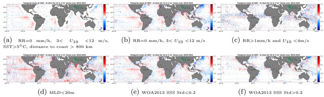
Figure 12: Temporal mean gridded over spatial boxes of size 1^\circ \times 1^\circ of \Delta SSS (SMOS SSS L2-AVERAGED v700 (ESA) - Argo) for 6 different subdatasets corresponding to:RR=0 mm/h, 3 < U_{10} < 12 m/s, SST >5^\circ C, distance to coast > 800 km (a), RR=0 mm/h, 3 < U_{10} < 12 m/s (b), RR >1 mm/h and U_{10} < 4 m/s (c),MLD <20 m (d),WOA2013 SSS Std <0.2 (e),WOA2013 SSS Std >0.2 (f).
