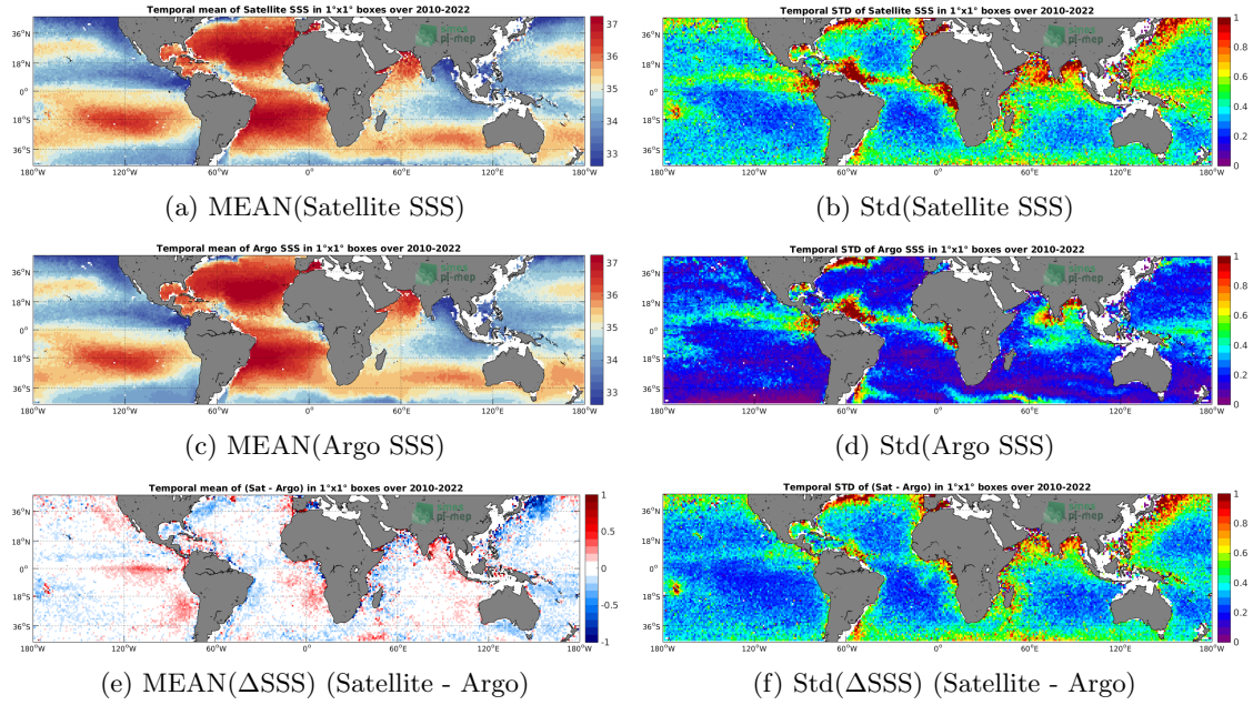
Figure 6: Temporal mean (left) and Std (right) of SSS from SMOS SSS L2-AVERAGED v700 (ESA) (top), Argo (middle), and of \Delta SSS (Satellite - Argo). Only match-up pairs are used to generate these maps.
