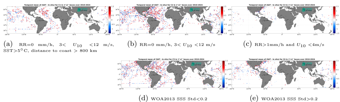
Figure 14: Temporal mean gridded over spatial boxes of size 1^\circ \times 1^\circ of \Delta\text{SSS} (SMOS SSS L2 v700 (ESA) - TSG (SAMOS)) for 5 different subdatasets corresponding to: RR=0 mm/h, 3 < U_{10} < 12 m/s, SST > 5°C, distance to coast > 800 km (a), RR=0 mm/h, 3 < U_{10} < 12 m/s (b), RR > 1mm/h and U_{10} < 4 m/s (c), WOA2013 SSS Std < 0.2 (d), WOA2013 SSS Std > 0.2 (e).
