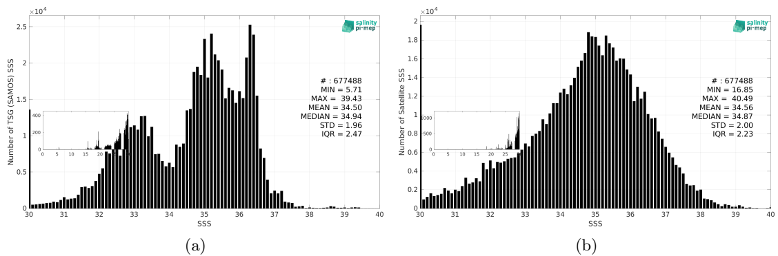
Figure 3: Histograms of SSS from TSG (SAMOS) (a) and SMOS SSS L2 v700 (ESA) (b) considering all match-up pairs per bins of 0.1 over the Mid-Low Latitudes 45N-45S Pi-MEP region and for the full satellite product period.
