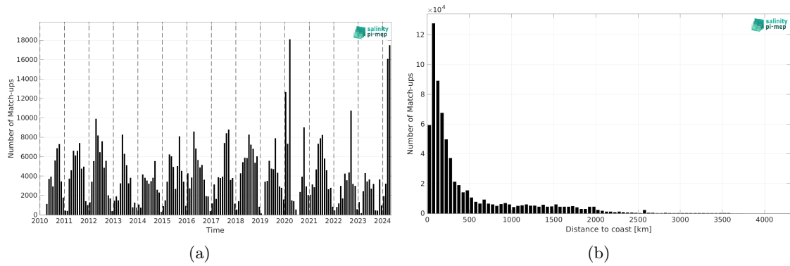
Figure 2: Number of match-ups between TSG (SAMOS) and SMOS SSS L2 v700 (ESA) SSS as a function of time (a) and as function of the distance to coast (b) over the Mid-Low Latitudes 45N-45S Pi-MEP region and for the full satellite product period.
