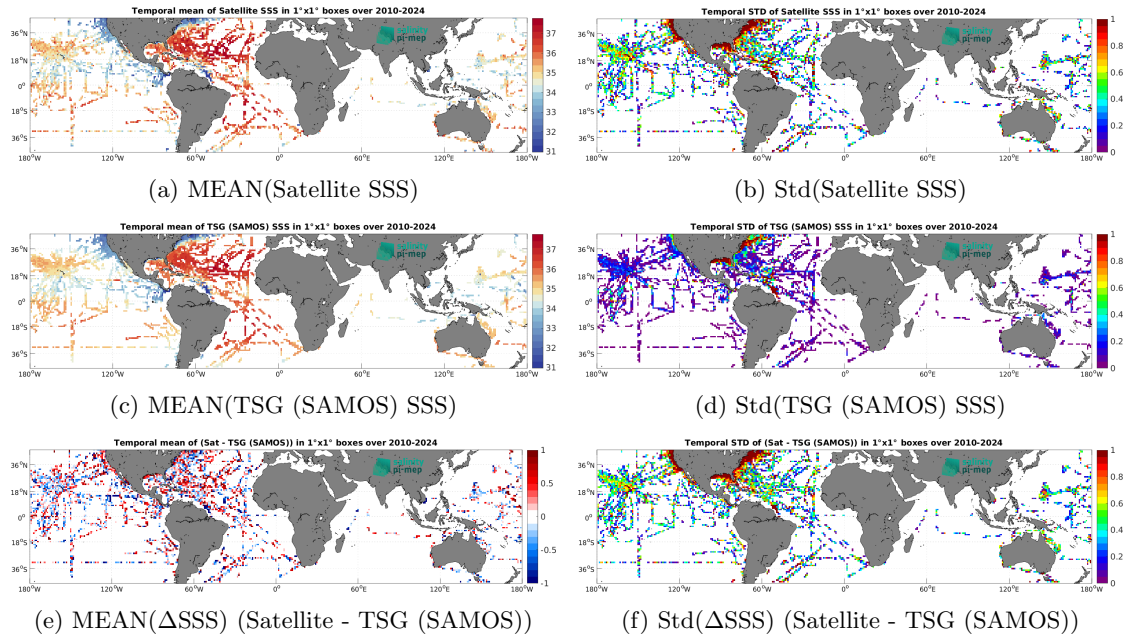
Figure 7: Temporal mean (left) and Std (right) of SSS from SMOS SSS L2 v700 (ESA) (top), TSG (SAMOS) (middle), and of \Delta SSS (Satellite - TSG (SAMOS)). Only match-up pairs are used to generate these maps.
