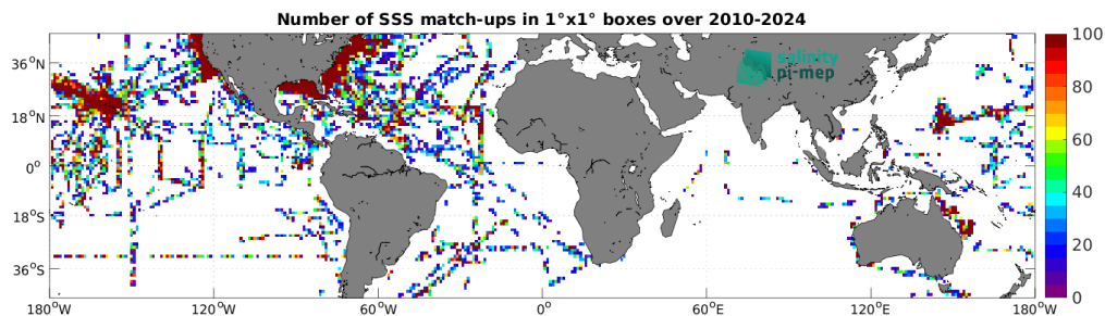
Figure 5: Number of SSS match-ups between TSG (SAMOS) SSS and the SMOS SSS L2 v700 (ESA) SSS product for the Mid-Low Latitudes 45N-45S Pi-MEP region over 1^\circ \times 1^\circ boxes and for the full satellite product period.
