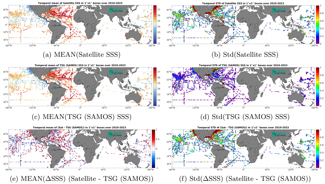
Figure 6: Temporal mean (left) and Std (right) of SSS from SMOS SSS L2 v700 (ESA) (top), TSG (SAMOS) (middle), and of \Delta SSS (Satellite - TSG (SAMOS)). Only match-up pairs are used to generate these maps.
