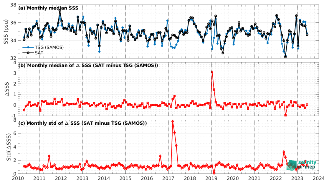
Figure 7: Time series of the monthly median SSS (top), median of \Delta SSS (Satellite - TSG (SAMOS)) and Std of \Delta SSS (Satellite - TSG (SAMOS)) over the Mid-Low Latitudes 45N-45S Pi-MEP region considering all match-ups collected by the Pi-MEP.
