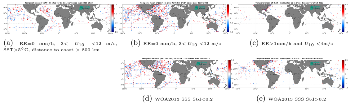
Figure 12: Temporal mean gridded over spatial boxes of size 1^\circ \times 1^\circ of \Delta SSS (SMOS SSS L2 v700 (ESA) - TSG (SAMOS)) for 5 different subdatasets corresponding to:RR=0 mm/h, 3 < U_{10} < 12 m/s, SST>5°C, distance to coast > 800 km (a), RR=0 mm/h, 3 < U_{10} < 12 m/s (b), RR>1mm/h and U_{10} < 4 m/s (c), WOA2013 SSS Std<0.2 (d), WOA2013 SSS Std>0.2 (e).
