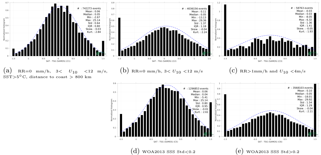
Figure 13: Normalized histogram of \Delta SSS (SMOS SSS L2 v700 (ESA) - TSG (SAMOS)) for 5 different subdatasets corresponding to: RR=0 mm/h, 3 < U_{10} < 12 m/s, SST >5^\circ\text{C} , distance to coast > 800 km (a), RR=0 mm/h, 3 < U_{10} < 12 m/s (b), RR >1 mm/h and U_{10} < 4 m/s (c), WOA2013 SSS Std <0.2 (d), WOA2013 SSS Std >0.2 (e).
