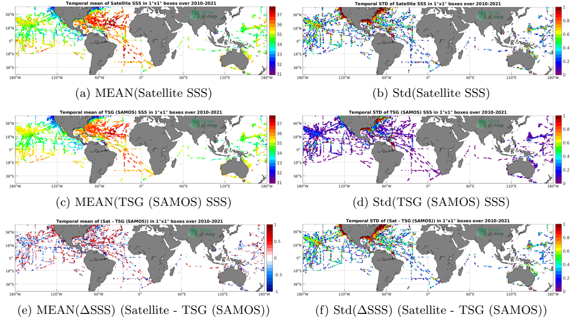
Figure 6: Temporal mean (left) and Std (right) of SSS from SMOS SSS L2 v700 (ESA) (top), TSG (SAMOS) (middle), and of \Delta SSS (Satellite - TSG (SAMOS)). Only match-up pairs are used to generate these maps.
