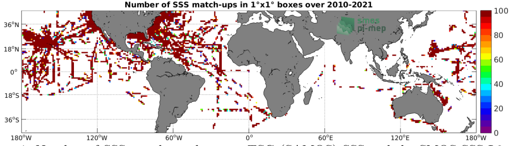
Figure 4: Number of SSS match-ups between TSG (SAMOS) SSS and the SMOS SSS L2 v700 (ESA) SSS product for the Mid-Low Latitudes 45N-45S Pi-MEP region over 1^\circ \times 1^\circ boxes and for the full satellite product period.
