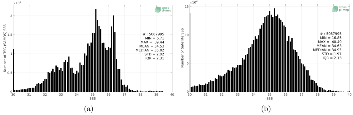
Figure 2: Histograms of SSS from TSG (SAMOS) (a) and SMOS SSS L2 v700 (ESA) (b) considering all match-up pairs per bins of 0.1 over the Mid-Low Latitudes 45N-45S Pi-MEP region and for the full satellite product period.
