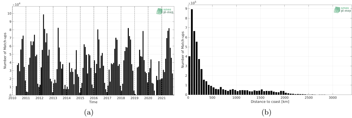
Figure 1: Number of match-ups between TSG (SAMOS) and SMOS SSS L2 v700 (ESA) SSS as a function of time (a) and as function of the distance to coast (b) over the Mid-Low Latitudes 45N-45S Pi-MEP region and for the full satellite product period.
