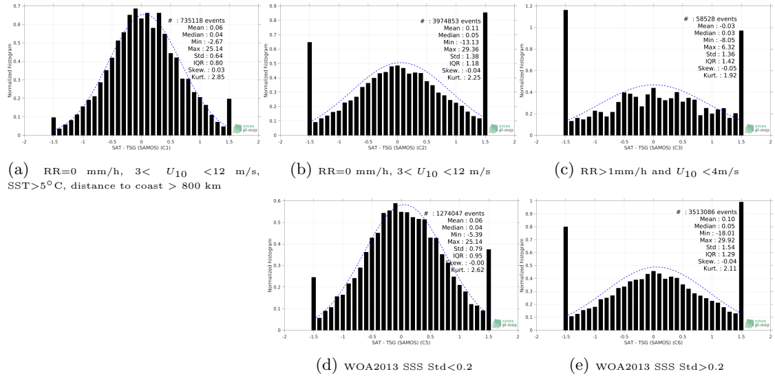
Figure 13: Normalized histogram of \Delta\text{SSS} (SMOS SSS L2 v700 (ESA) - TSG (SAMOS)) for 5 different subdatasets corresponding to: \text{RR}=0 mm/h, 3 < U_{10} < 12 m/s, \text{SST}>5^\circ\text{C} , distance to coast > 800 km (a), \text{RR}=0 mm/h, 3 < U_{10} < 12 m/s (b), \text{RR}>1\text{mm/h} and U_{10} < 4\text{m/s} (c), WOA2013 SSS Std <0.2 (d), WOA2013 SSS Std >0.2 (e).
