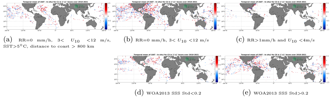
Figure 12: Temporal mean gridded over spatial boxes of size 1^\circ \times 1^\circ of \Delta\text{SSS} (SMOS SSS L2 v700 (ESA) - TSG (SAMOS)) for 5 different subdatasets corresponding to: \text{RR}=0 mm/h, 3 < U_{10} < 12 m/s, \text{SST}>5^\circ\text{C} , distance to coast > 800 km (a), \text{RR}=0 mm/h, 3 < U_{10} < 12 m/s (b), \text{RR}>1\text{mm/h} and U_{10} < 4\text{m/s} (c), WOA2013 SSS Std <0.2 (d), WOA2013 SSS Std >0.2 (e).
