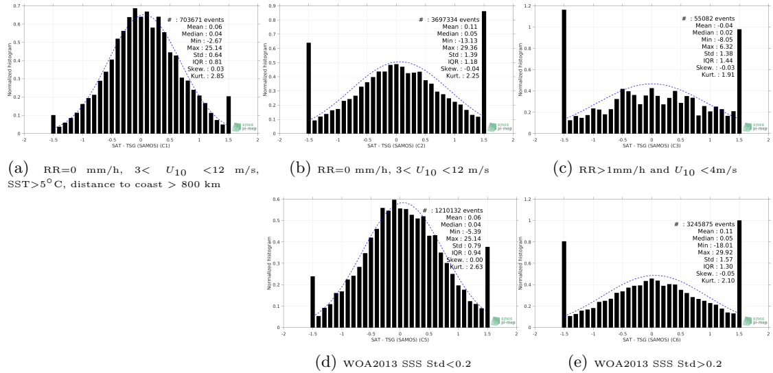
Figure 13: Normalized histogram of \Delta SSS (SMOS SSS L2 v700 (ESA) - TSG (SAMOS)) for 5 different subdatasets corresponding to: RR=0 mm/h, 3 < U_{10} < 12 m/s, SST > 5^\circ C , distance to coast > 800 km (a), RR=0 mm/h, 3 < U_{10} < 12 m/s (b), RR > 1 mm/h and U_{10} < 4 m/s (c), WOA2013 SSS Std < 0.2 (d), WOA2013 SSS Std > 0.2 (e).
