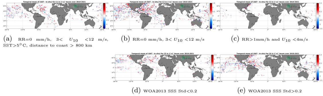
Figure 12: Temporal mean gridded over spatial boxes of size 1^\circ \times 1^\circ of \Delta SSS (SMOS SSS L2 v700 (ESA) - TSG (SAMOS)) for 5 different subdatasets corresponding to: RR=0 mm/h, 3 < U_{10} < 12 m/s, SST > 5^\circ C , distance to coast > 800 km (a), RR=0 mm/h, 3 < U_{10} < 12 m/s (b), RR > 1 mm/h and U_{10} < 4 m/s (c), WOA2013 SSS Std < 0.2 (d), WOA2013 SSS Std > 0.2 (e).
