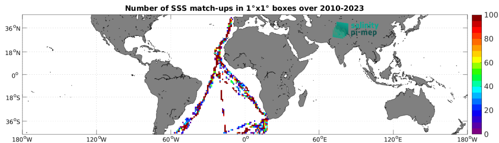
Figure 5: Number of SSS match-ups between TSG (Polarstern) SSS and the SMOS SSS L2 v700 (ESA) SSS product for the Mid-Low Latitudes 45N-45S Pi-MEP region over 1^\circ \times 1^\circ boxes and for the full satellite product period.
