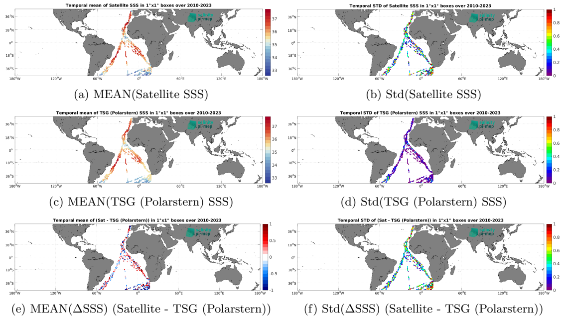
Figure 7: Temporal mean (left) and Std (right) of SSS from SMOS SSS L2 v700 (ESA) (top), TSG (Polarstern) (middle), and of \Delta SSS (Satellite - TSG (Polarstern)). Only match-up pairs are used to generate these maps.
