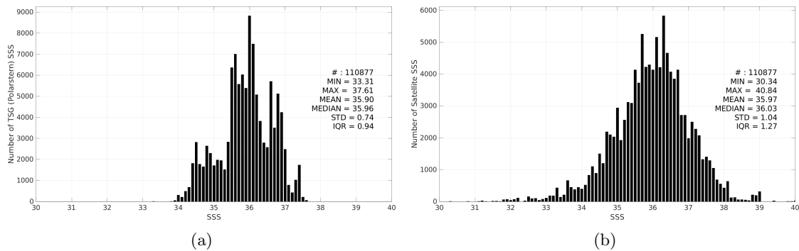
Figure 3: Histograms of SSS from TSG (Polarstern) (a) and SMOS SSS L2 v700 (ESA) (b) considering all match-up pairs per bins of 0.1 over the Mid-Low Latitudes 45N-45S Pi-MEP region and for the full satellite product period.
