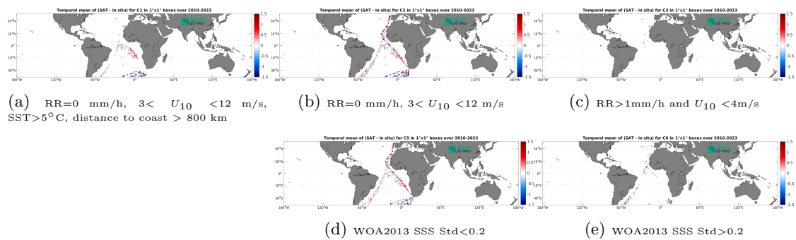
Figure 14: Temporal mean gridded over spatial boxes of size 1^\circ \times 1^\circ of \Delta SSS (SMOS SSS L2 v700 (ESA) - TSG (Polarstern)) for 5 different subdatasets corresponding to: RR=0 mm/h, 3 < U_{10} < 12 m/s, SST > 5°C, distance to coast > 800 km (a), RR=0 mm/h, 3 < U_{10} < 12 m/s (b), RR > 1mm/h and U_{10} < 4 m/s (c), WOA2013 SSS Std < 0.2 (d), WOA2013 SSS Std > 0.2 (e).
