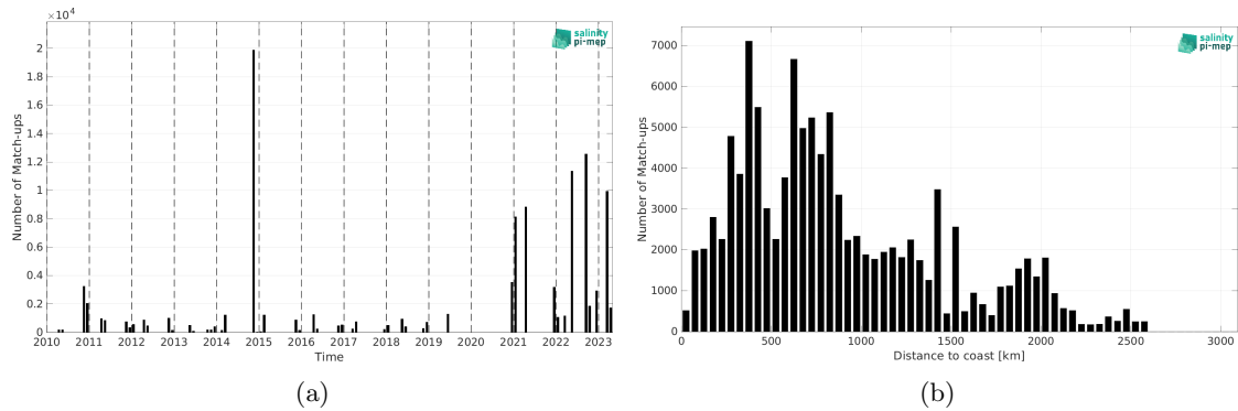
Figure 2: Number of match-ups between TSG (Polarstern) and SMOS SSS L2 v700 (ESA) SSS as a function of time (a) and as function of the distance to coast (b) over the Mid-Low Latitudes 45N-45S Pi-MEP region and for the full satellite product period.
