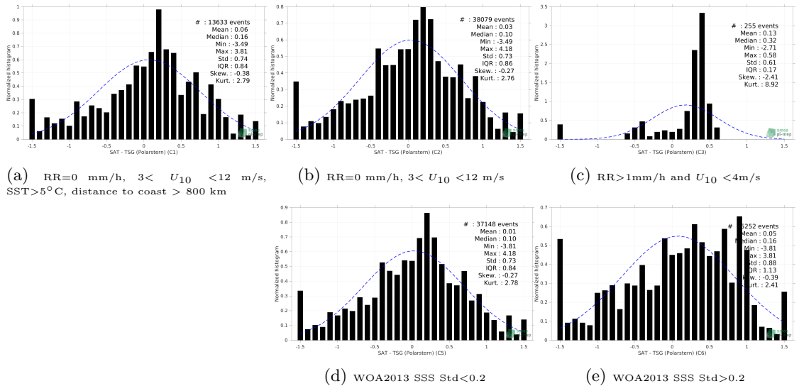
Figure 13: Normalized histogram of \Delta SSS (SMOS SSS L2 v700 (ESA) - TSG (Polarstern)) for 5 different subdatasets corresponding to: RR=0 mm/h, 3 < U_{10} < 12 m/s, SST >5^\circ\text{C} , distance to coast > 800 km (a), RR=0 mm/h, 3 < U_{10} < 12 m/s (b), RR >1 mm/h and U_{10} < 4 m/s (c), WOA2013 SSS Std <0.2 (d), WOA2013 SSS Std >0.2 (e).
