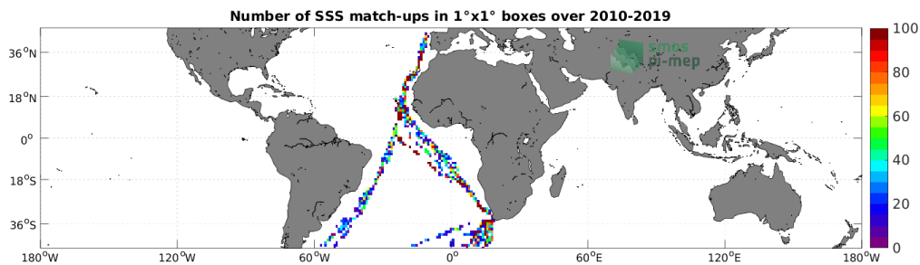
Figure 4: Number of SSS match-ups between TSG (Polarstern) SSS and the SMOS SSS L2 v700 (ESA) SSS product for the Mid-Low Latitudes 45N-45S Pi-MEP region over 1^\circ \times 1^\circ boxes and for the full satellite product period.
