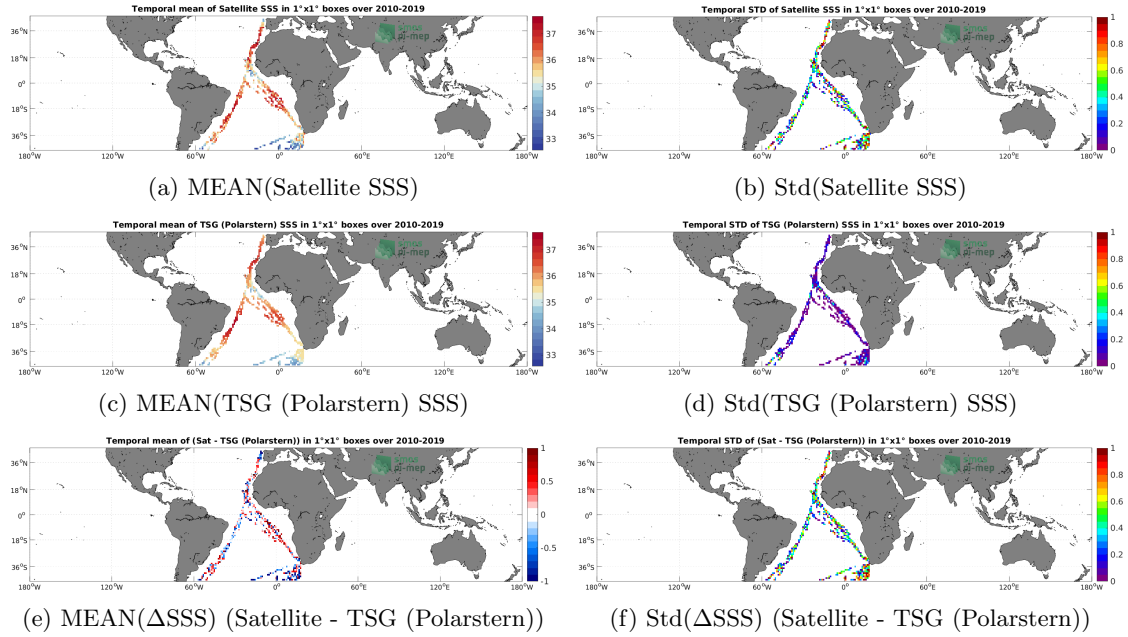
Figure 6: Temporal mean (left) and Std (right) of SSS from SMOS SSS L2 v700 (ESA) (top), TSG (Polarstern) (middle), and of \Delta SSS (Satellite - TSG (Polarstern)). Only match-up pairs are used to generate these maps.
