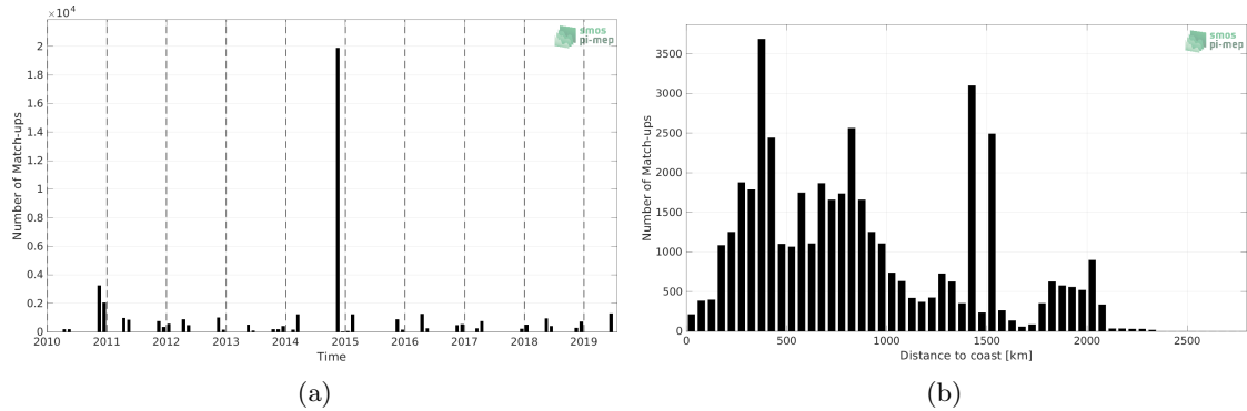
Figure 1: Number of match-ups between TSG (Polarstern) and SMOS SSS L2 v700 (ESA) SSS as a function of time (a) and as function of the distance to coast (b) over the Mid-Low Latitudes 45N-45S Pi-MEP region and for the full satellite product period.
