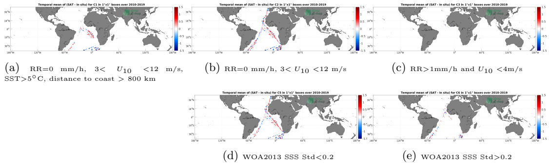
Figure 12: Temporal mean gridded over spatial boxes of size 1^\circ \times 1^\circ of \Delta SSS (SMOS SSS L2 v700 (ESA) - TSG (Polarstern)) for 5 different subdatasets corresponding to:RR=0 mm/h, 3 < U_{10} < 12 m/s, SST >5^\circ\text{C} , distance to coast > 800 km (a), RR=0 mm/h, 3 < U_{10} < 12 m/s (b), RR >1 mm/h and U_{10} < 4 m/s (c), WOA2013 SSS Std <0.2 (d), WOA2013 SSS Std >0.2 (e).
