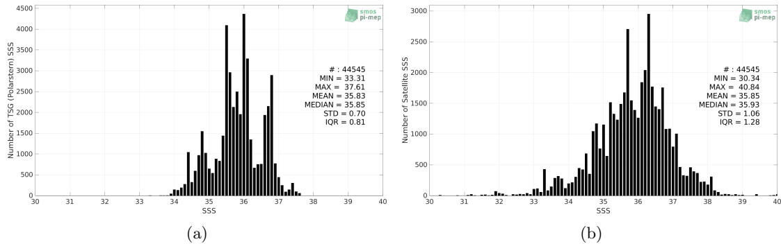
Figure 2: Histograms of SSS from TSG (Polarstern) (a) and SMOS SSS L2 v700 (ESA) (b) considering all match-up pairs per bins of 0.1 over the Mid-Low Latitudes 45N-45S Pi-MEP region and for the full satellite product period.
