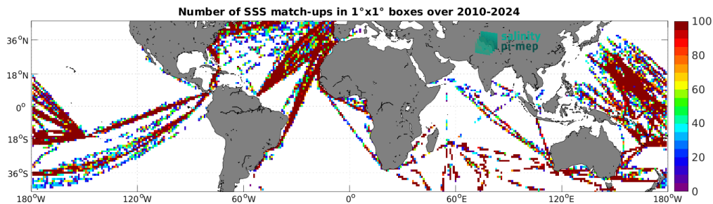
Figure 5: Number of SSS match-ups between TSG (LEGOS-DM) SSS and the SMOS SSS L2 v700 (ESA) SSS product for the Mid-Low Latitudes 45N-45S Pi-MEP region over 1°×1° boxes and for the full satellite product period.
