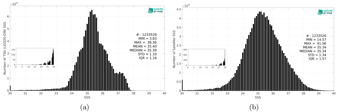
Figure 3: Histograms of SSS from TSG (LEGOS-DM) (a) and SMOS SSS L2 v700 (ESA) (b) considering all match-up pairs per bins of 0.1 over the Mid-Low Latitudes 45N-45S Pi-MEP region and for the full satellite product period.
