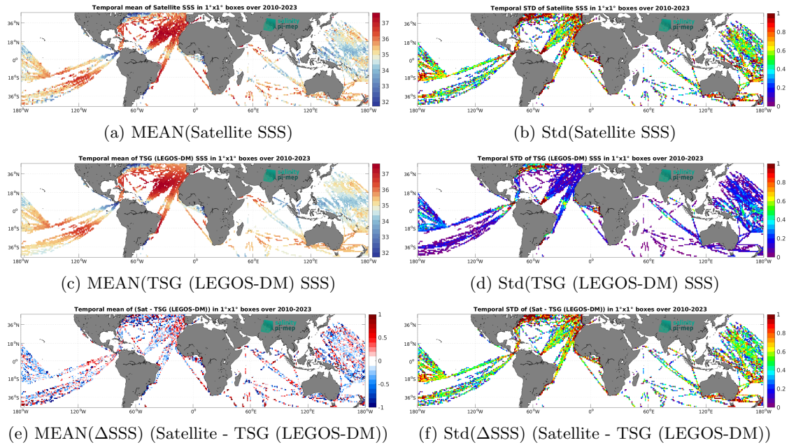
Figure 7: Temporal mean (left) and Std (right) of SSS from SMOS SSS L2 v700 (ESA) (top), TSG (LEGOS-DM) (middle), and of \Delta SSS (Satellite - TSG (LEGOS-DM)). Only match-up pairs are used to generate these maps.
