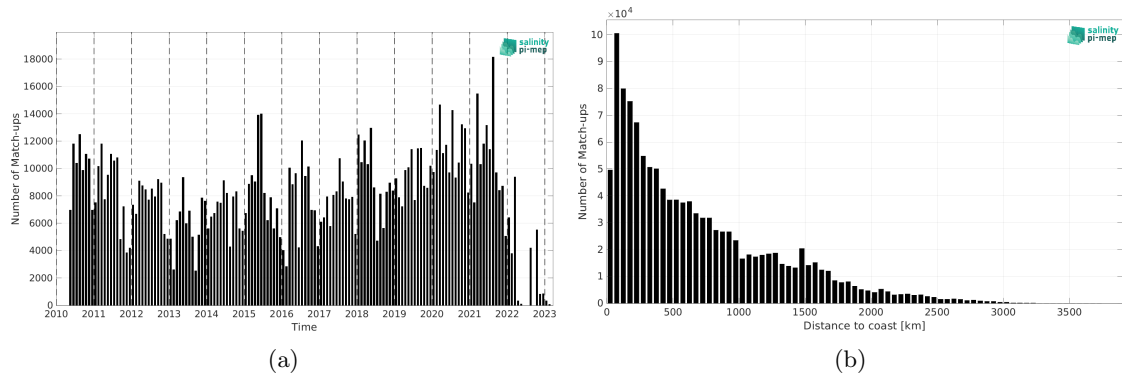
Figure 2: Number of match-ups between TSG (LEGOS-DM) and SMOS SSS L2 v700 (ESA) SSS as a function of time (a) and as function of the distance to coast (b) over the Mid-Low Latitudes 45N-45S Pi-MEP region and for the full satellite product period.
