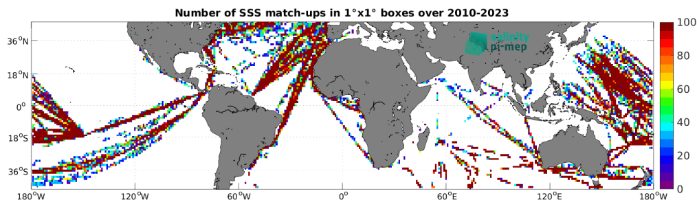
Figure 5: Number of SSS match-ups between TSG (LEGOS-DM) SSS and the SMOS SSS L2 v700 (ESA) SSS product for the Mid-Low Latitudes 45N-45S Pi-MEP region over 1^\circ \times 1^\circ boxes and for the full satellite product period.
