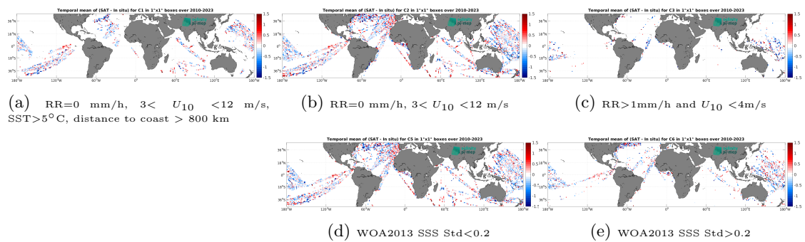
Figure 14: Temporal mean gridded over spatial boxes of size 1^\circ \times 1^\circ of \Delta\text{SSS} (SMOS SSS L2 v700 (ESA) - TSG (LEGOS-DM)) for 5 different subdatasets corresponding to:RR=0 mm/h, 3 < U_{10} < 12 m/s, SST>5°C, distance to coast > 800 km (a), RR=0 mm/h, 3 < U_{10} < 12 m/s (b), RR>1mm/h and U_{10} < 4 m/s (c), WOA2013 SSS Std<0.2 (d), WOA2013 SSS Std>0.2 (e).
