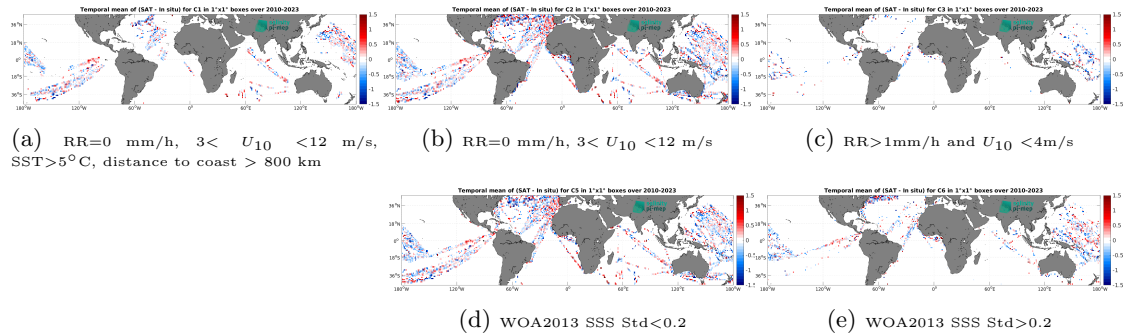
Figure 12: Temporal mean gridded over spatial boxes of size 1^\circ \times 1^\circ of \Delta SSS (SMOS SSS L2 v700 (ESA) - TSG (LEGOS-DM)) for 5 different subdatasets corresponding to:RR=0 mm/h, 3 < U_{10} < 12 m/s, SST>5°C, distance to coast > 800 km (a), RR=0 mm/h, 3 < U_{10} < 12 m/s (b), RR>1mm/h and U_{10} < 4 m/s (c), WOA2013 SSS Std<0.2 (d), WOA2013 SSS Std>0.2 (e).
