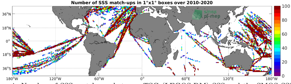
Figure 4: Number of SSS match-ups between TSG (LEGOS-DM) SSS and the SMOS SSS L2 v700 (ESA) SSS product for the Mid-Low Latitudes 45N-45S Pi-MEP region over 1^\circ \times 1^\circ boxes and for the full satellite product period.
