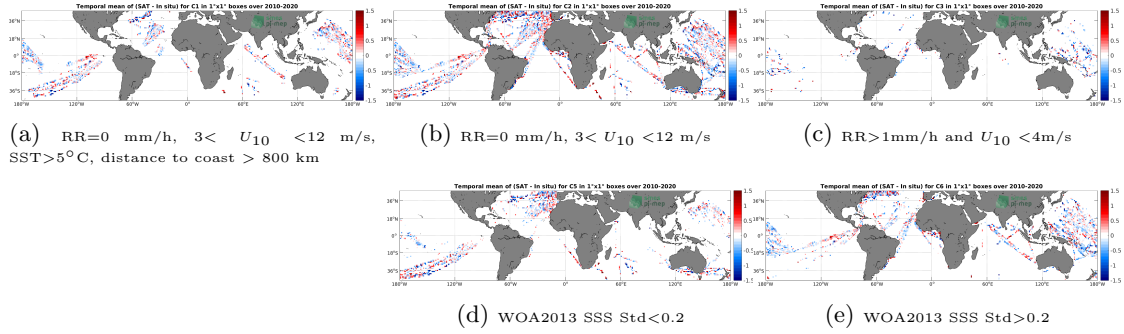
Figure 12: Temporal mean gridded over spatial boxes of size 1^\circ \times 1^\circ of \Delta\text{SSS} (SMOS SSS L2 v700 (ESA) - TSG (LEGOS-DM)) for 5 different subdatasets corresponding to: RR=0 mm/h, 3 < U_{10} < 12 m/s, SST >5^\circ\text{C} , distance to coast > 800 km (a), RR=0 mm/h, 3 < U_{10} < 12 m/s (b), RR >1 mm/h and U_{10} < 4 m/s (c), WOA2013 SSS Std <0.2 (d), WOA2013 SSS Std >0.2 (e).
