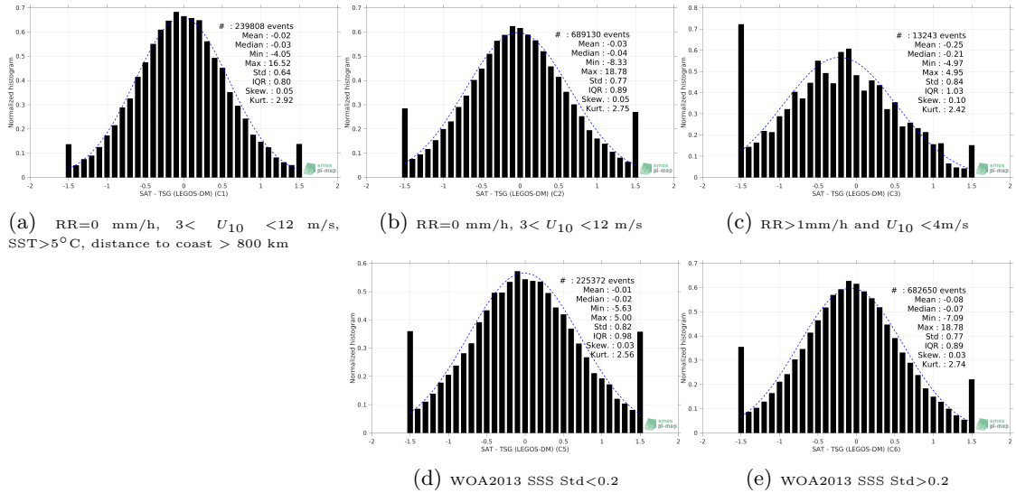
Figure 13: Normalized histogram of \Delta\text{SSS} (SMOS SSS L2 v700 (ESA) - TSG (LEGOS-DM)) for 5 different subdatasets corresponding to: RR=0 mm/h, 3 < U_{10} < 12 m/s, SST >5^\circ\text{C} , distance to coast > 800 km (a), RR=0 mm/h, 3 < U_{10} < 12 m/s (b), RR >1 mm/h and U_{10} < 4 m/s (c), WOA2013 SSS Std <0.2 (d), WOA2013 SSS Std >0.2 (e).
