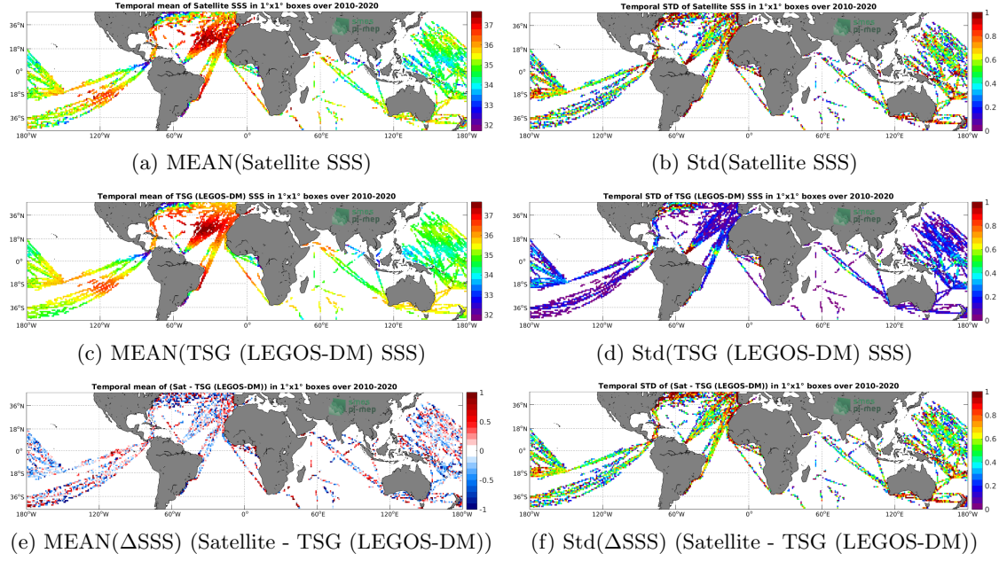
Figure 6: Temporal mean (left) and Std (right) of SSS from SMOS SSS L2 v700 (ESA) (top), TSG (LEGOS-DM) (middle), and of \Delta SSS (Satellite - TSG (LEGOS-DM)). Only match-up pairs are used to generate these maps.
