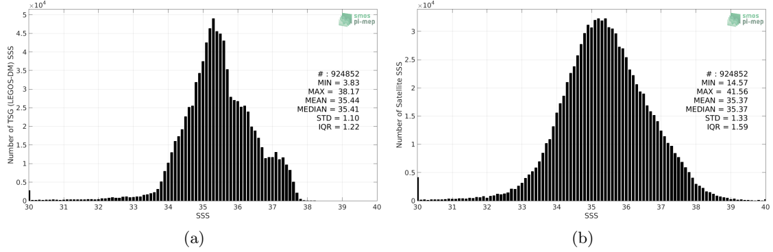
Figure 2: Histograms of SSS from TSG (LEGOS-DM) (a) and SMOS SSS L2 v700 (ESA) (b) considering all match-up pairs per bins of 0.1 over the Mid-Low Latitudes 45N-45S Pi-MEP region and for the full satellite product period.
