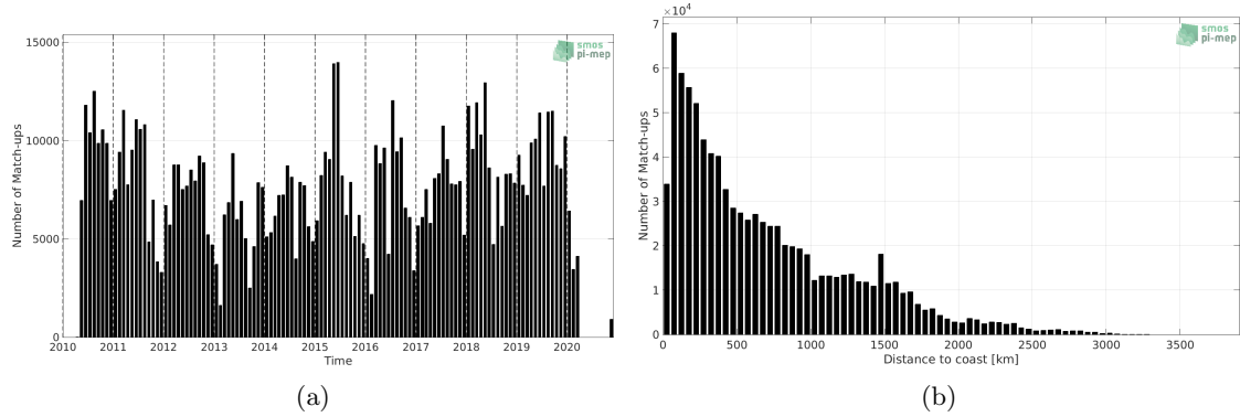
Figure 1: Number of match-ups between TSG (LEGOS-DM) and SMOS SSS L2 v700 (ESA) SSS as a function of time (a) and as function of the distance to coast (b) over the Mid-Low Latitudes 45N-45S Pi-MEP region and for the full satellite product period.
