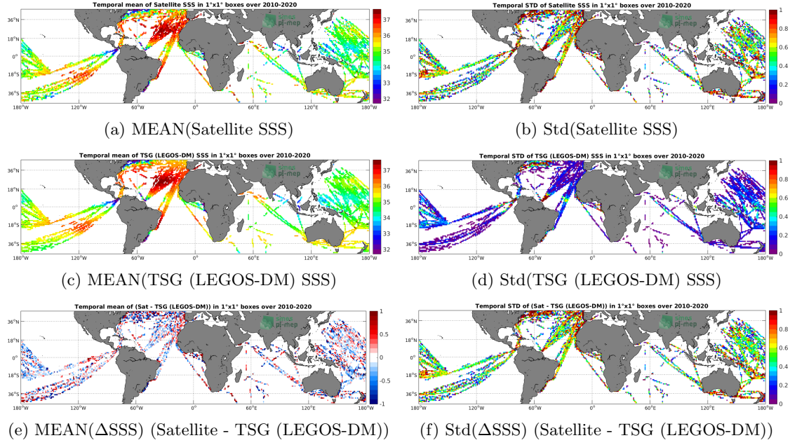
Figure 6: Temporal mean (left) and Std (right) of SSS from SMOS SSS L2 v700 (ESA) (top), TSG (LEGOS-DM) (middle), and of \Delta SSS (Satellite - TSG (LEGOS-DM)). Only match-up pairs are used to generate these maps.
