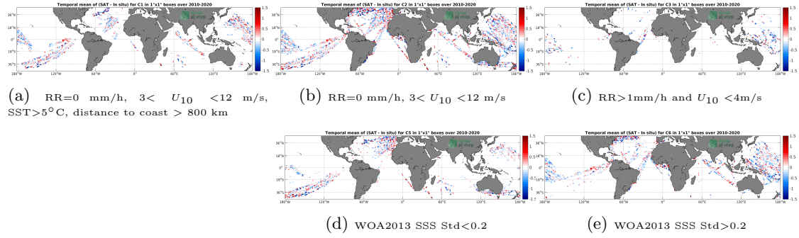
Figure 12: Temporal mean gridded over spatial boxes of size 1^\circ \times 1^\circ of \Delta SSS (SMOS SSS L2 v700 (ESA) - TSG (LEGOS-DM)) for 5 different subdatasets corresponding to: RR=0 mm/h, 3 < U_{10} < 12 m/s, SST > 5^\circ C , distance to coast > 800 km (a), RR=0 mm/h, 3 < U_{10} < 12 m/s (b), RR > 1 mm/h and U_{10} < 4 m/s (c), WOA2013 SSS Std < 0.2 (d), WOA2013 SSS Std > 0.2 (e).
