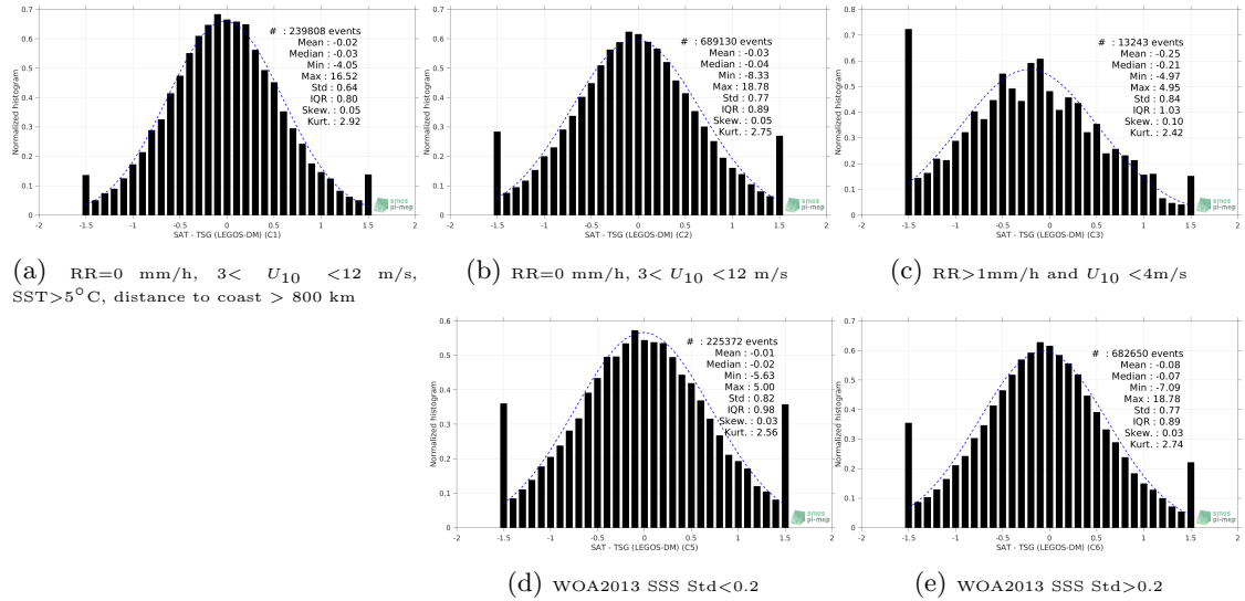
Figure 13: Normalized histogram of \Delta SSS (SMOS SSS L2 v700 (ESA) - TSG (LEGOS-DM)) for 5 different subdatasets corresponding to: RR=0 mm/h, 3 < U_{10} < 12 m/s, SST > 5^\circ C , distance to coast > 800 km (a), RR=0 mm/h, 3 < U_{10} < 12 m/s (b), RR > 1 mm/h and U_{10} < 4 m/s (c), WOA2013 SSS Std < 0.2 (d), WOA2013 SSS Std > 0.2 (e).
