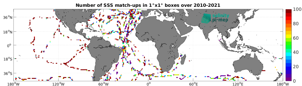
Figure 5: Number of SSS match-ups between TSG (GOSUD-Sailing-ship) SSS and the SMOS SSS L2 v700 (ESA) SSS product for the Mid-Low Latitudes 45N-45S Pi-MEP region over 1^\circ \times 1^\circ boxes and for the full satellite product period.
