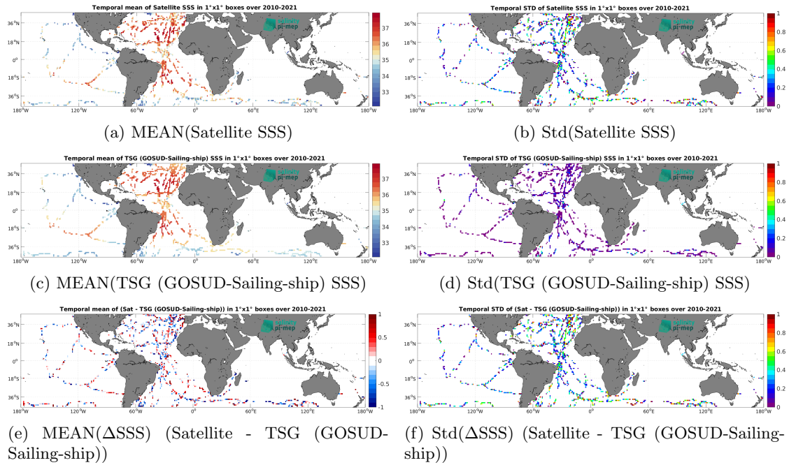
Figure 7: Temporal mean (left) and Std (right) of SSS from SMOS SSS L2 v700 (ESA) (top), TSG (GOSUD-Sailing-ship) (middle), and of \Delta SSS (Satellite - TSG (GOSUD-Sailing-ship)). Only match-up pairs are used to generate these maps.
