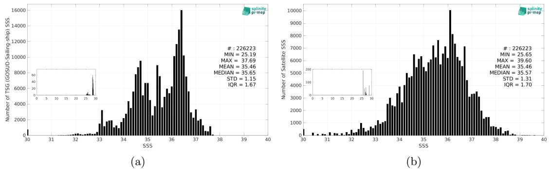
Figure 3: Histograms of SSS from TSG (GOSUD-Sailing-ship) (a) and SMOS SSS L2 v700 (ESA) (b) considering all match-up pairs per bins of 0.1 over the Mid-Low Latitudes 45N-45S Pi-MEP region and for the full satellite product period.
