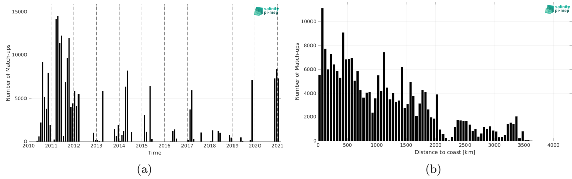
Figure 2: Number of match-ups between TSG (GOSUD-Sailing-ship) and SMOS SSS L2 v700 (ESA) SSS as a function of time (a) and as function of the distance to coast (b) over the Mid-Low Latitudes 45N-45S Pi-MEP region and for the full satellite product period.
