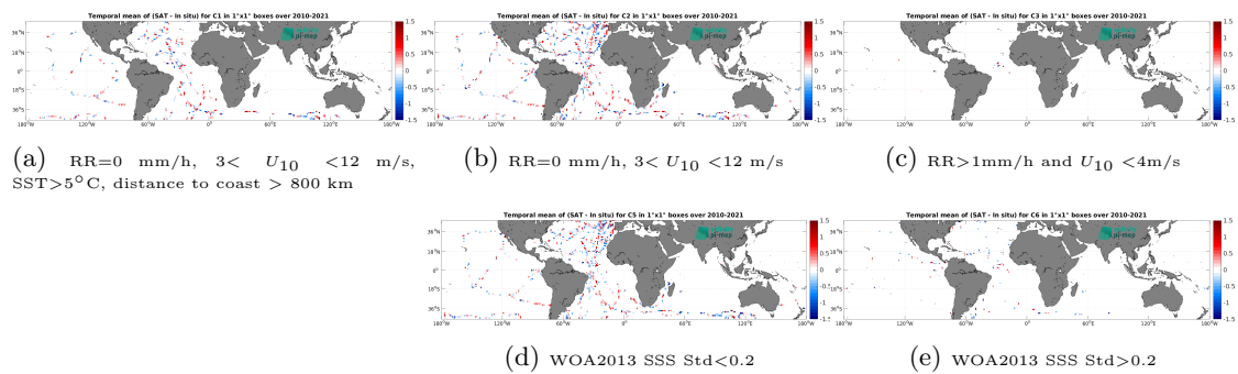
Figure 14: Temporal mean gridded over spatial boxes of size 1^\circ \times 1^\circ of \Delta SSS (SMOS SSS L2 v700 (ESA) - TSG (GOSUD-Sailing-ship)) for 5 different subdatasets corresponding to:RR=0 mm/h, 3 < U_{10} < 12 m/s, SST>5°C, distance to coast > 800 km (a), RR=0 mm/h, 3 < U_{10} < 12 m/s (b), RR>1mm/h and U_{10} < 4 m/s (c), WOA2013 SSS Std<0.2 (d), WOA2013 SSS Std>0.2 (e).
