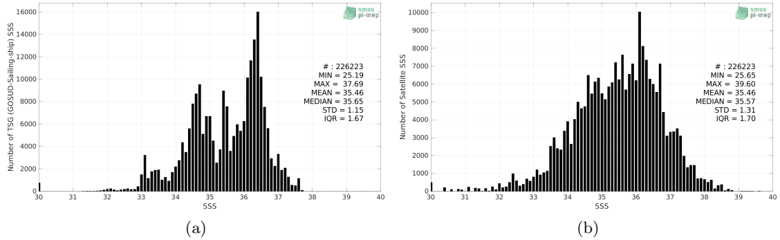
Figure 2: Histograms of SSS from TSG (GOSUD-Sailing-ship) (a) and SMOS SSS L2 v700 (ESA) (b) considering all match-up pairs per bins of 0.1 over the Mid-Low Latitudes 45N-45S Pi-MEP region and for the full satellite product period.
