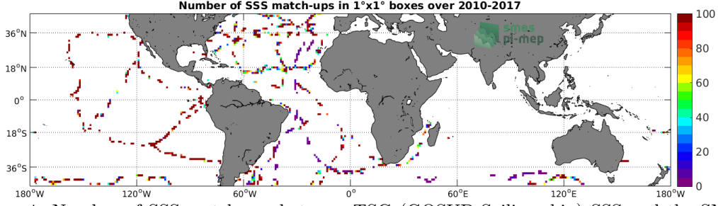
Figure 4: Number of SSS match-ups between TSG (GOSUD-Sailing-ship) SSS and the SMOS SSS L2 v700 (ESA) SSS product for the Mid-Low Latitudes 45N-45S Pi-MEP region over 1^\circ \times 1^\circ boxes and for the full satellite product period.
