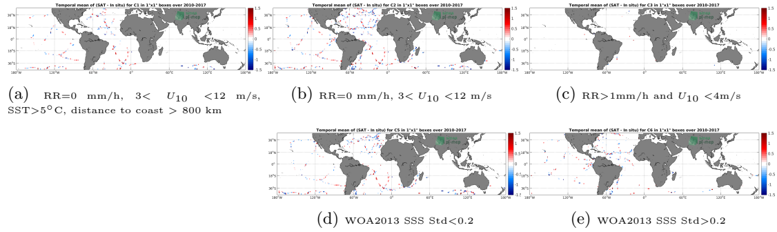
Figure 12: Temporal mean gridded over spatial boxes of size 1^\circ \times 1^\circ of \Delta SSS (SMOS SSS L2 v700 (ESA) - TSG (GOSUD-Sailing-ship)) for 5 different subdatasets corresponding to: RR=0 mm/h, 3 < U_{10} < 12 m/s, SST > 5^\circ C , distance to coast > 800 km (a), RR=0 mm/h, 3 < U_{10} < 12 m/s (b), RR > 1 mm/h and U_{10} < 4 m/s (c), WOA2013 SSS Std < 0.2 (d), WOA2013 SSS Std > 0.2 (e).
