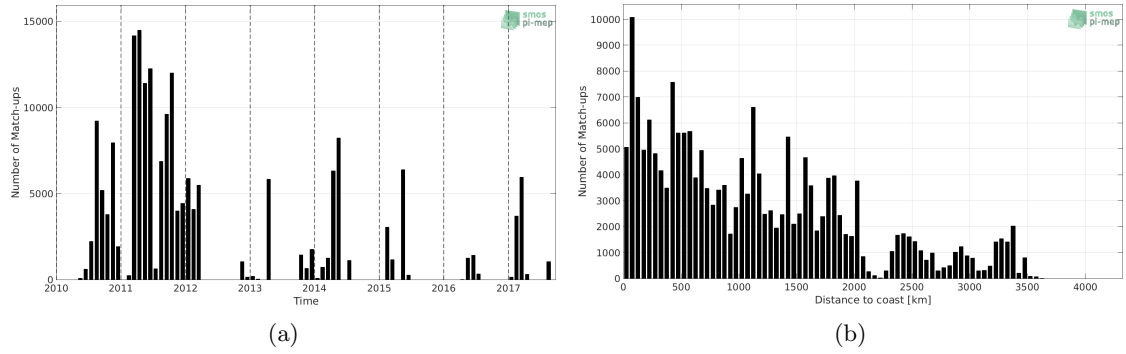
Figure 1: Number of match-ups between TSG (GOSUD-Sailing-ship) and SMOS SSS L2 v700 (ESA) SSS as a function of time (a) and as function of the distance to coast (b) over the Mid-Low Latitudes 45N-45S Pi-MEP region and for the full satellite product period.
