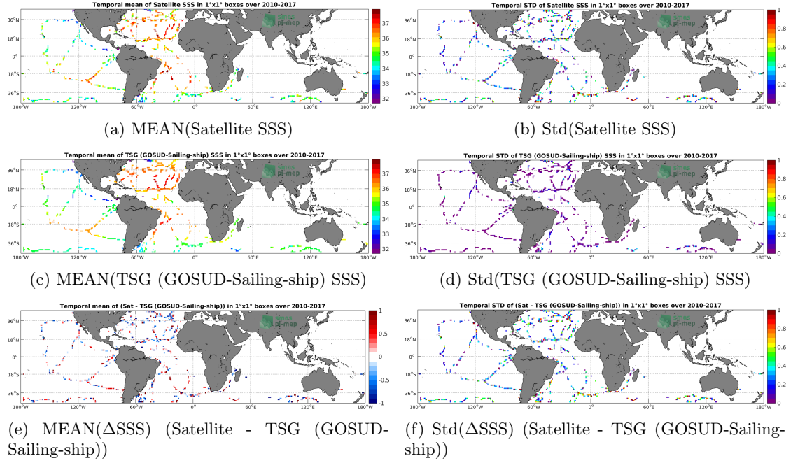
Figure 6: Temporal mean (left) and Std (right) of SSS from SMOS SSS L2 v700 (ESA) (top), TSG (GOSUD-Sailing-ship) (middle), and of \Delta SSS (Satellite - TSG (GOSUD-Sailing-ship)). Only match-up pairs are used to generate these maps.
