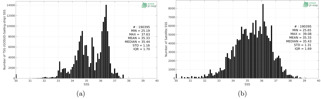
Figure 2: Histograms of SSS from TSG (GOSUD-Sailing-ship) (a) and SMOS SSS L2 v700 (ESA) (b) considering all match-up pairs per bins of 0.1 over the Mid-Low Latitudes 45N-45S Pi-MEP region and for the full satellite product period.
