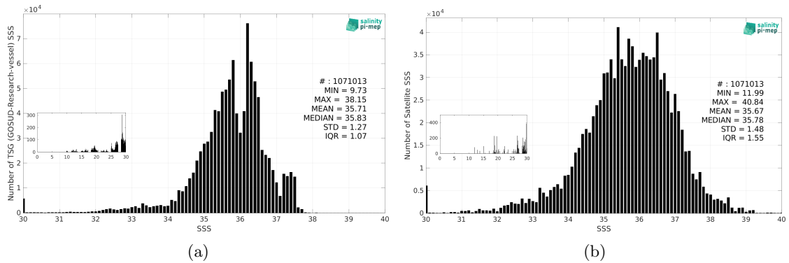
Figure 3: Histograms of SSS from TSG (GOSUD-Research-vessel) (a) and SMOS SSS L2 v700 (ESA) (b) considering all match-up pairs per bins of 0.1 over the Mid-Low Latitudes 45N-45S Pi-MEP region and for the full satellite product period.
