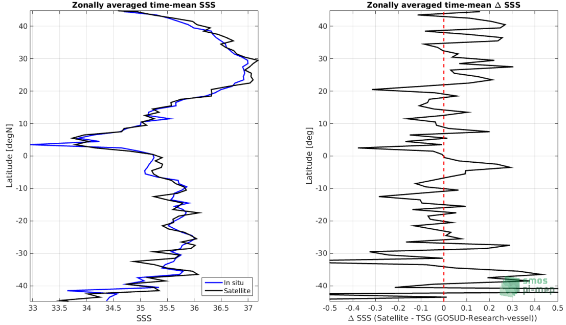
Figure 8: Left panel: Zonal mean SSS from SMOS SSS L2 v700 (ESA) satellite product (black) and from TSG (GOSUD-Research-vessel) (blue). Right panel: Zonal mean of \Delta SSS (Satellite - TSG (GOSUD-Research-vessel)) for all the collected Pi-MEP match-up pairs estimated over the full satellite product period.
