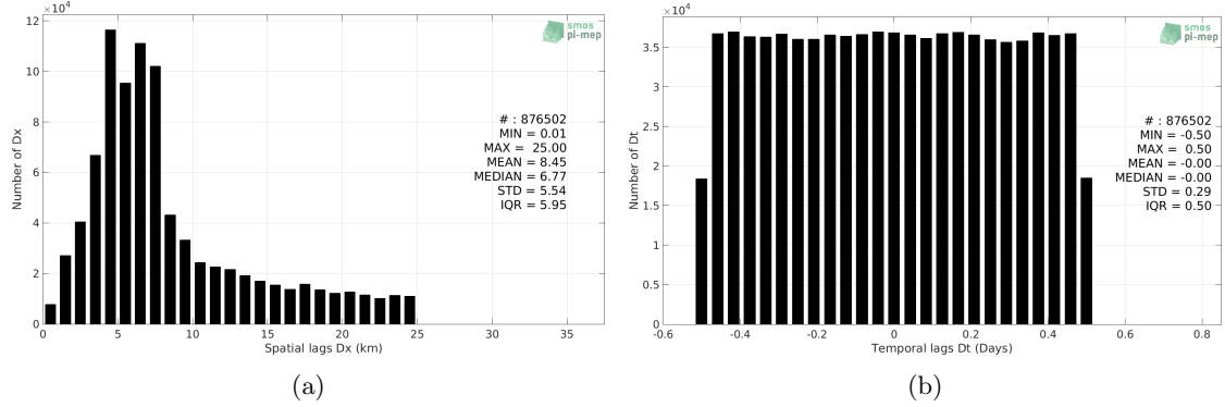
Figure 5: Histograms of the spatial (a) and temporal (b) lags between the location/time of the TSG (GOSUD-Research-vessel) measurement and the date of the corresponding SMOS SSS L2 v700 (ESA) SSS pixel.
