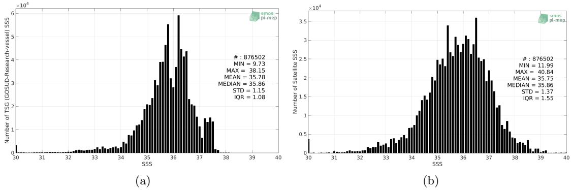
Figure 2: Histograms of SSS from TSG (GOSUD-Research-vessel) (a) and SMOS SSS L2 v700 (ESA) (b) considering all match-up pairs per bins of 0.1 over the Mid-Low Latitudes 45N-45S Pi-MEP region and for the full satellite product period.
