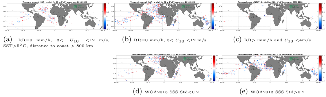
Figure 12: Temporal mean gridded over spatial boxes of size 1^\circ \times 1^\circ of \Delta SSS (SMOS SSS L2 v700 (ESA) - TSG (GOSUD-Research-vessel)) for 5 different subdatasets corresponding to: RR=0 mm/h, 3 < U_{10} < 12 m/s, SST > 5^\circ C , distance to coast > 800 km (a), RR=0 mm/h, 3 < U_{10} < 12 m/s (b), RR > 1 mm/h and U_{10} < 4 m/s (c), WOA2013 SSS Std < 0.2 (d), WOA2013 SSS Std > 0.2 (e).
