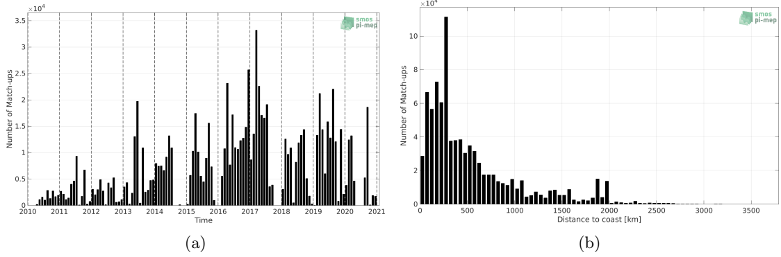
Figure 1: Number of match-ups between TSG (GOSUD-Research-vessel) and SMOS SSS L2 v700 (ESA) SSS as a function of time (a) and as function of the distance to coast (b) over the Mid-Low Latitudes 45N-45S Pi-MEP region and for the full satellite product period.
