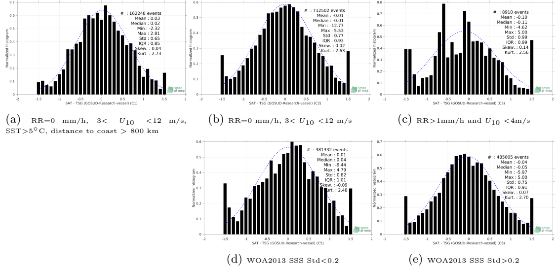
Figure 13: Normalized histogram of \Delta SSS (SMOS SSS L2 v700 (ESA) - TSG (GOSUD-Research-vessel)) for 5 different subdatasets corresponding to: RR=0 mm/h, 3 < U_{10} < 12 m/s, SST>5°C, distance to coast > 800 km (a), RR=0 mm/h, 3 < U_{10} < 12 m/s (b), RR>1mm/h and U_{10} < 4 m/s (c), WOA2013 SSS Std<0.2 (d), WOA2013 SSS Std>0.2 (e).
