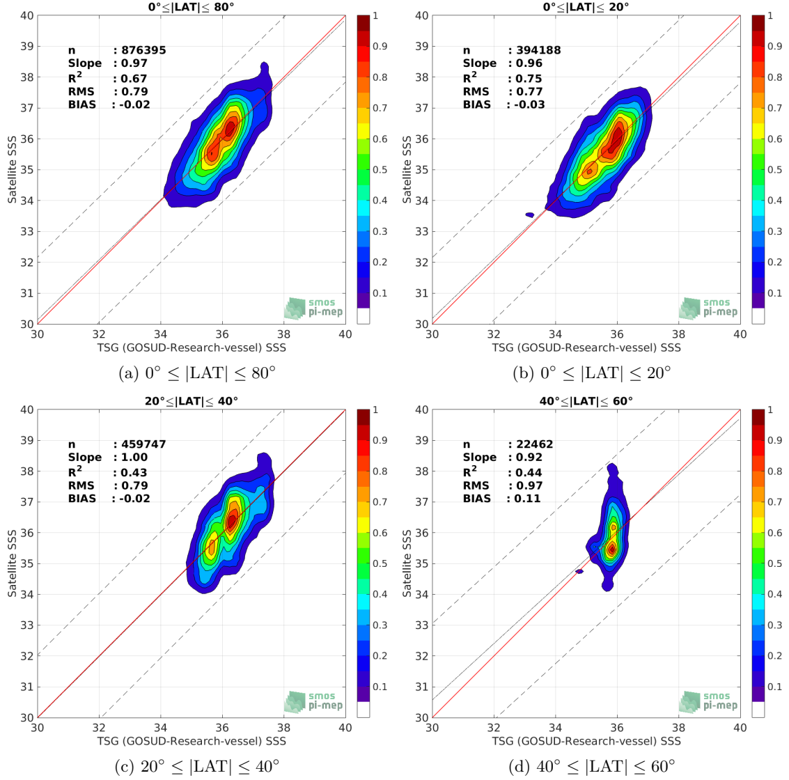
Figure 9: Contour maps of the concentration of SMOS SSS L2 v700 (ESA) SSS (y-axis) versus TSG (GOSUD-Research-vessel) SSS (x-axis) at match-up pairs for different latitude bands. For each plot, the red line shows x=y . The black thin and dashed lines indicate a linear fit through the data cloud and the \pm 95\% confidence levels, respectively. The number match-up pairs n , the slope and R^2 coefficient of the linear fit, the root mean square (RMS) and the mean bias between satellite and in situ data are indicated for each latitude band in each plots.
