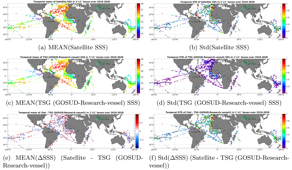
Figure 6: Temporal mean (left) and Std (right) of SSS from SMOS SSS L2 v700 (ESA) (top), TSG (GOSUD-Research-vessel) (middle), and of \Delta SSS (Satellite - TSG (GOSUD-Research-vessel)). Only match-up pairs are used to generate these maps.
