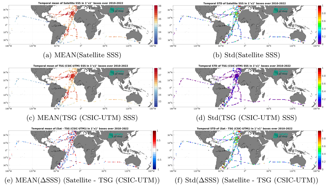
Figure 6: Temporal mean (left) and Std (right) of SSS from SMOS SSS L2 v700 (ESA) (top), TSG (CSIC-UTM) (middle), and of \Delta SSS (Satellite - TSG (CSIC-UTM)). Only match-up pairs are used to generate these maps.
