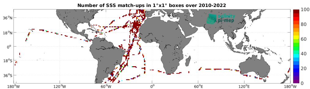
Figure 4: Number of SSS match-ups between TSG (CSIC-UTM) SSS and the SMOS SSS L2 v700 (ESA) SSS product for the Mid-Low Latitudes 45N-45S Pi-MEP region over 1^\circ \times 1^\circ boxes and for the full satellite product period.
