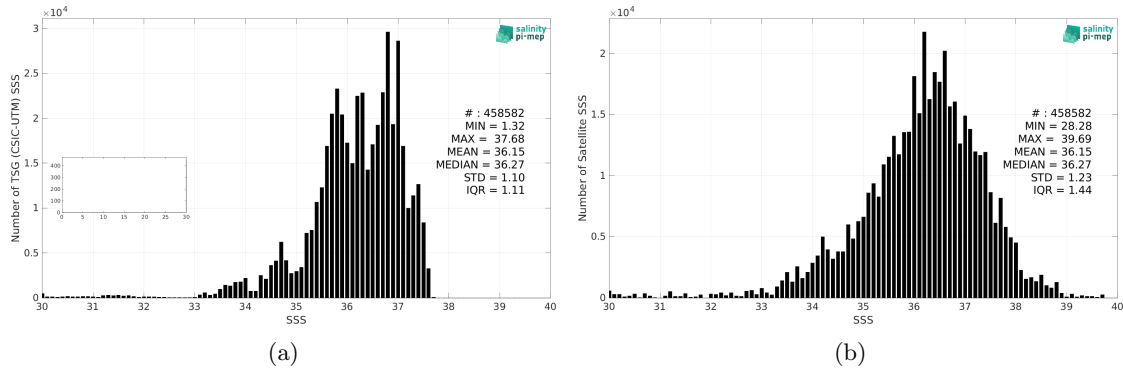
Figure 2: Histograms of SSS from TSG (CSIC-UTM) (a) and SMOS SSS L2 v700 (ESA) (b) considering all match-up pairs per bins of 0.1 over the Mid-Low Latitudes 45N-45S Pi-MEP region and for the full satellite product period.
