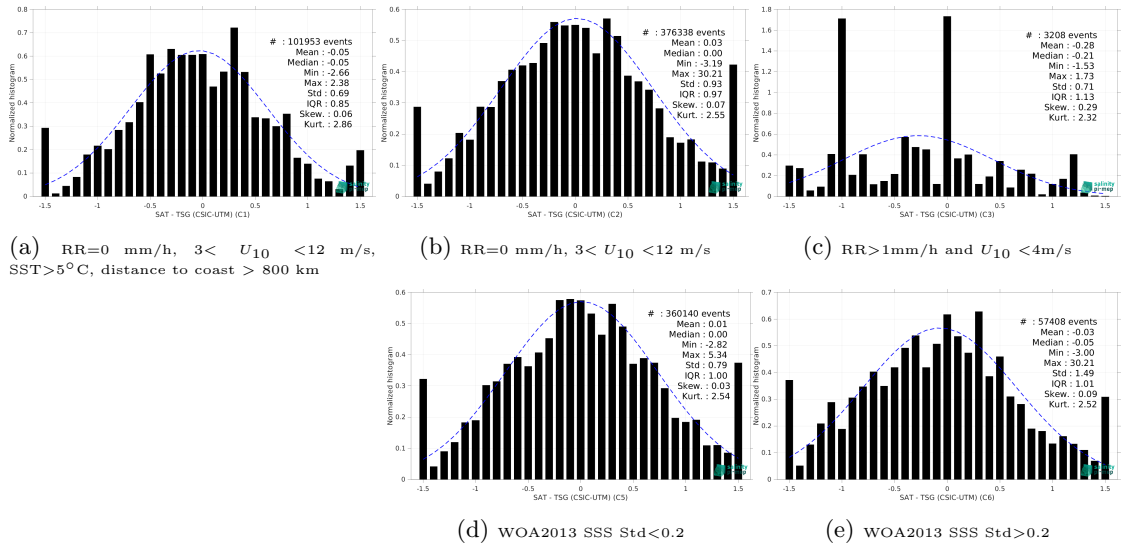
Figure 13: Normalized histogram of \Delta SSS (SMOS SSS L2 v700 (ESA) - TSG (CSIC-UTM)) for 5 different subdatasets corresponding to: RR=0 mm/h, 3 < U_{10} < 12 m/s, SST>5°C, distance to coast > 800 km (a), RR=0 mm/h, 3 < U_{10} < 12 m/s (b), RR>1mm/h and U_{10} < 4 m/s (c), WOA2013 SSS Std<0.2 (d), WOA2013 SSS Std>0.2 (e).
