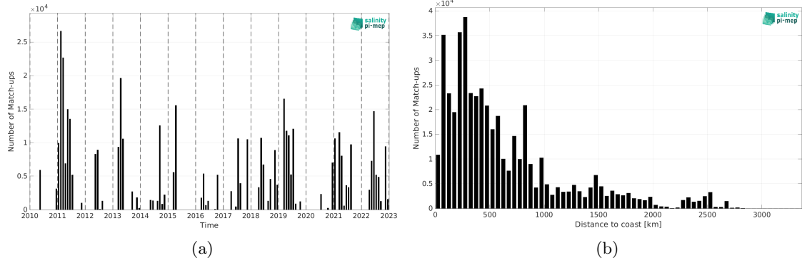
Figure 1: Number of match-ups between TSG (CSIC-UTM) and SMOS SSS L2 v700 (ESA) SSS as a function of time (a) and as function of the distance to coast (b) over the Mid-Low Latitudes 45N-45S Pi-MEP region and for the full satellite product period.
